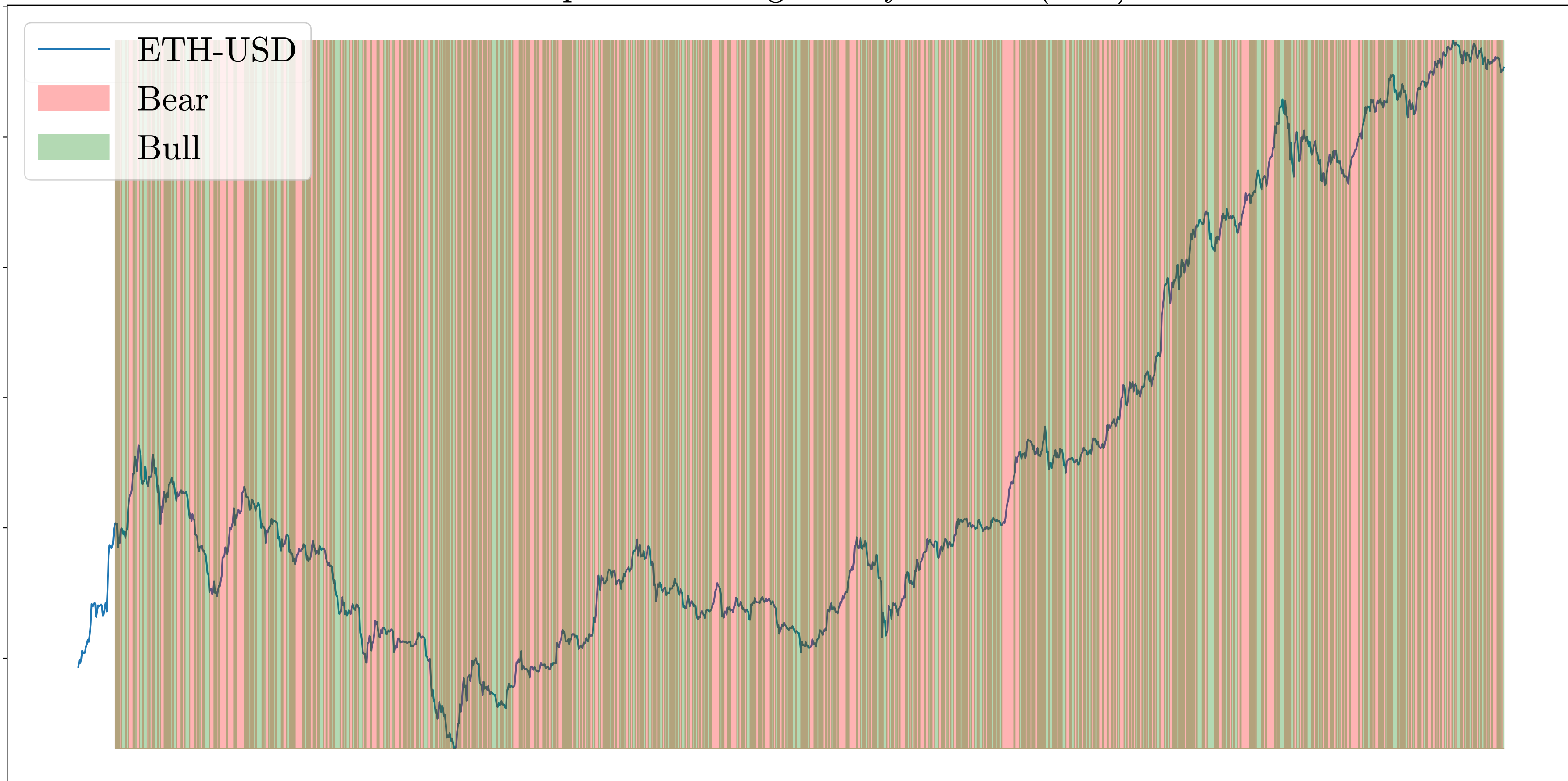
In-Sample Fitted Regimes by the JM ( \lambda=0 )
