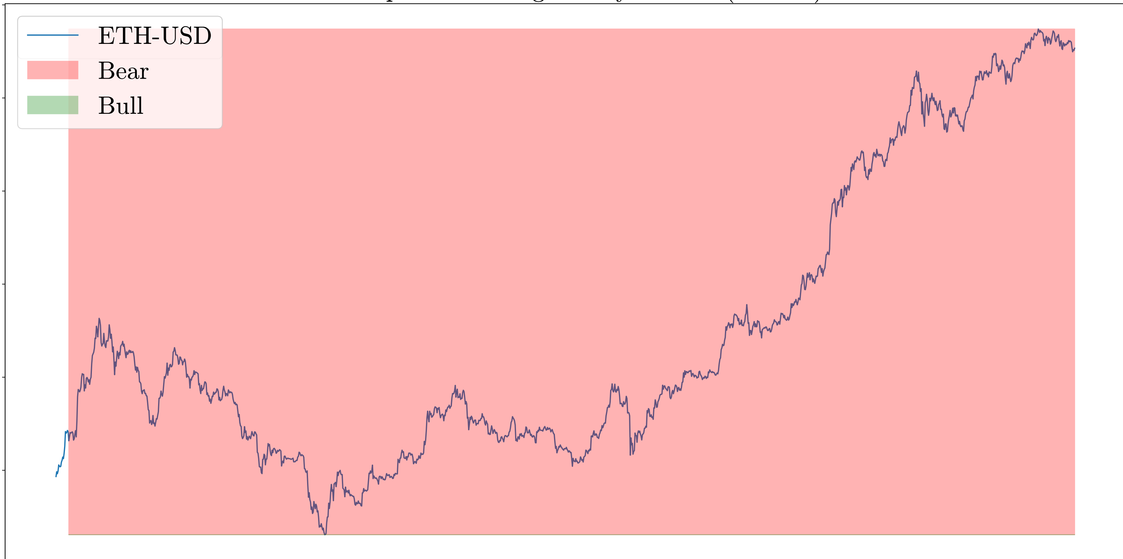
In-Sample Fitted Regimes by the JM ( \lambda=10.0 )
