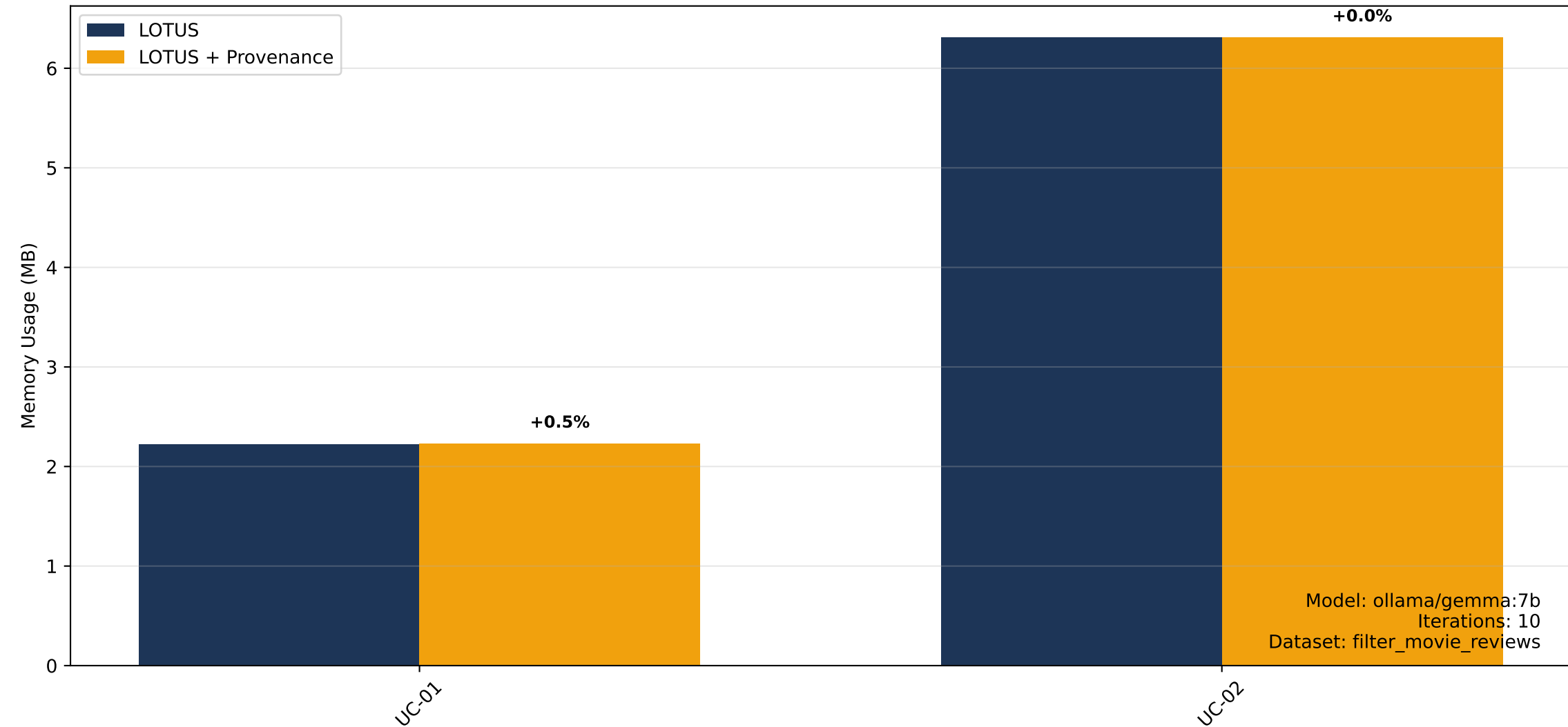
Benchmarking Memory Usage (MB) for LOTUS Pipelines
