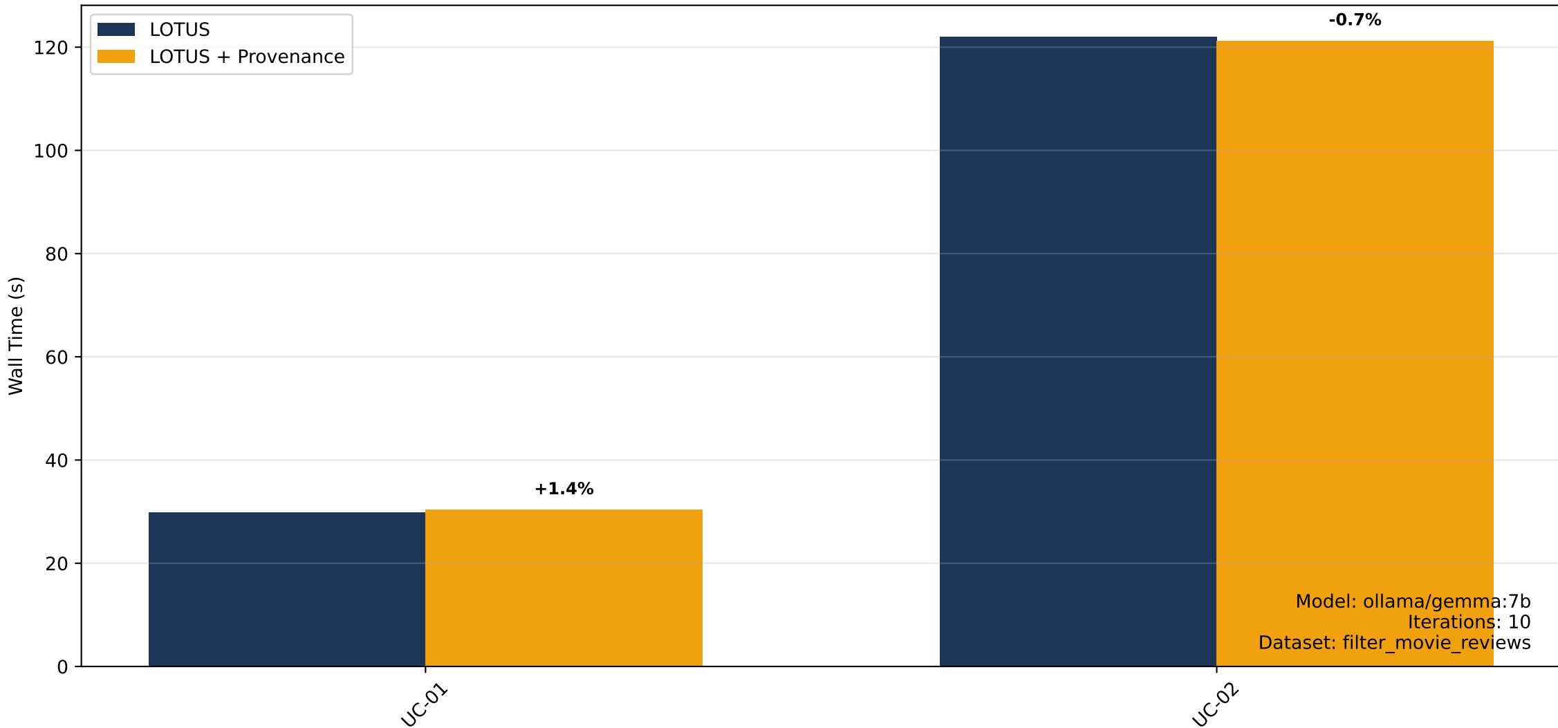
Benchmarking Wall Time (s) for LOTUS Pipelines
