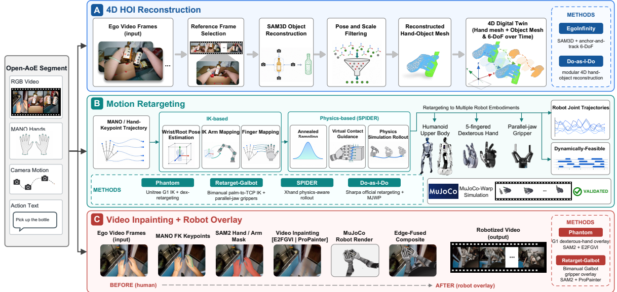
Figure 4: Reconstruction and Retargeting. A smartphone-captured AoE egocentric video can be projected into three complementary outputs: 4D hand-object interaction assets, robot-usable motion, and robotized video. The toolchain integrates EgoInfinity and Do-as-I-Do for 4D reconstruction; Phantom, Retarget-Galbot, SPIDER/XHand, and Do-as-I-Do/Sharpa for motion retargeting; and Phantom or Retarget-Galbot for SAM2-based video inpainting and MuJoCo robot overlay.
