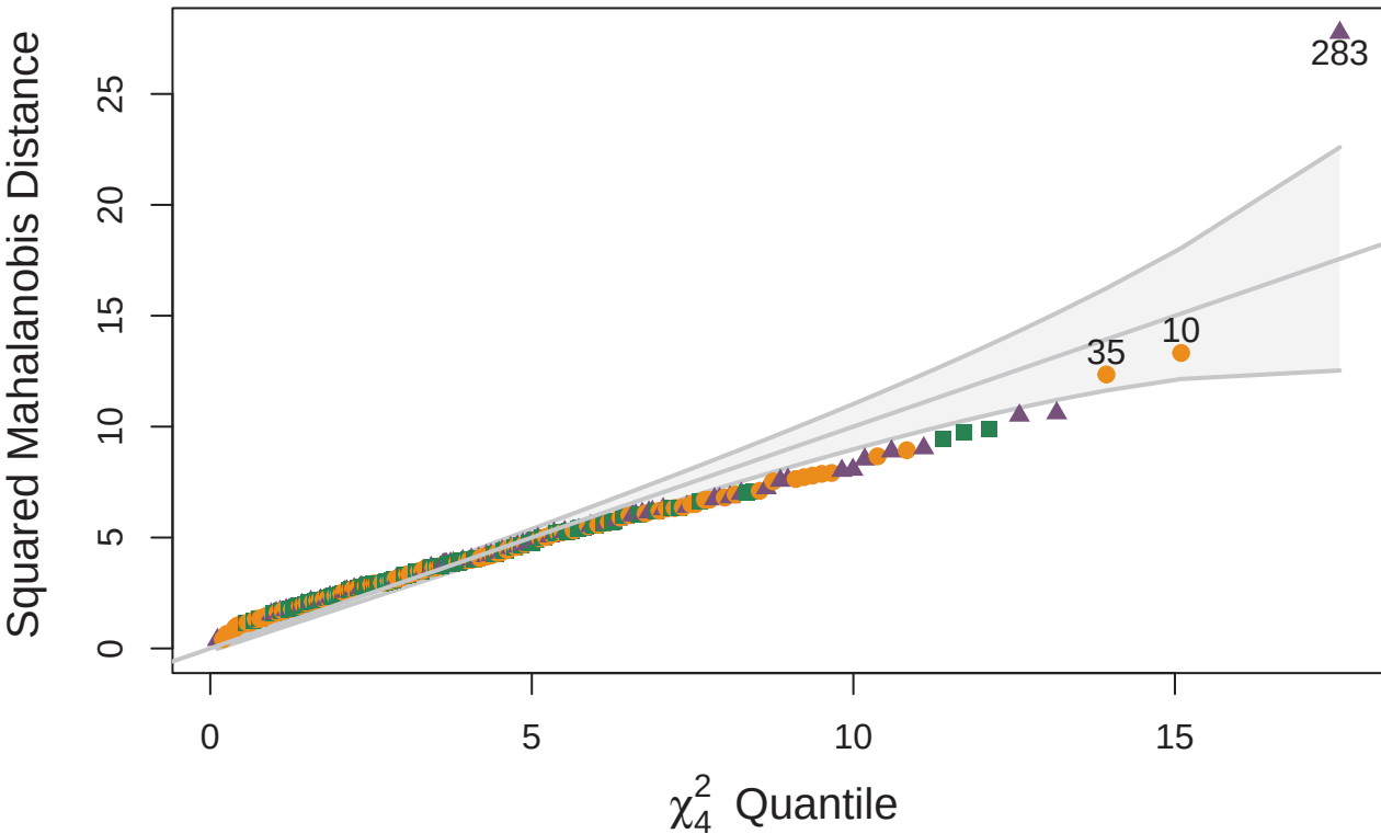
Chi-Square Q-Q Plot of Penguin numeric variables
