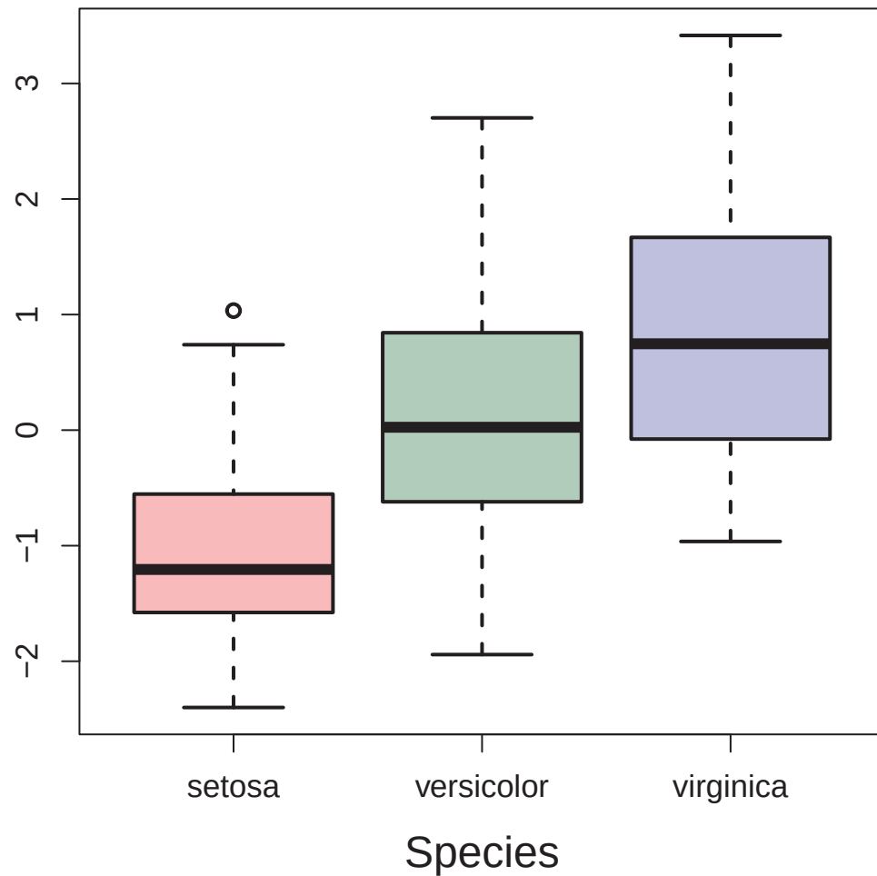
Canonical scores
