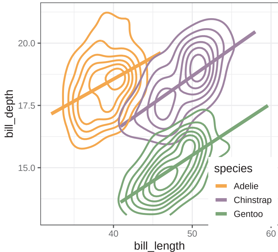
geom_density_2d
