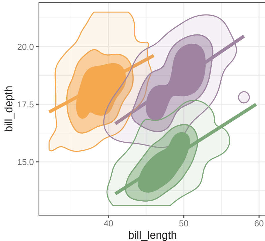
ggdensity::geom_hdr
