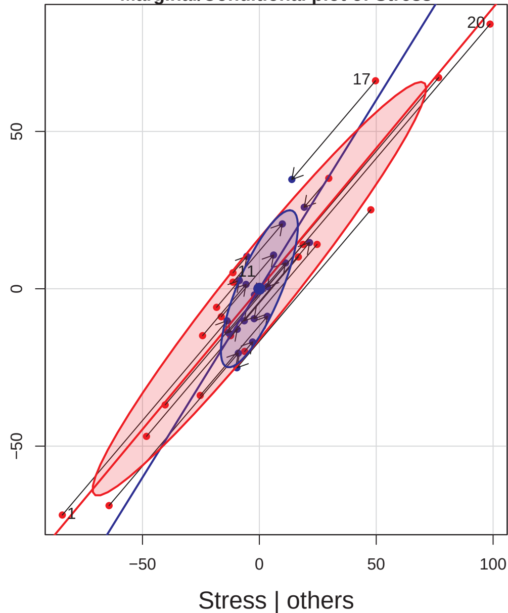
Marginal/Conditional plot of Stress
