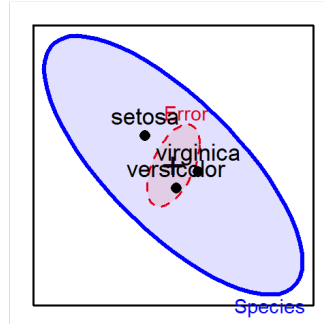
heplot(mod) 2D HE plot for two responses
