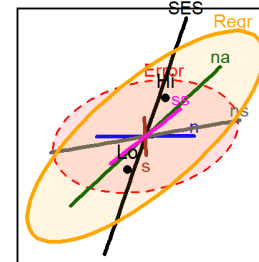
heplot(mod, hypotheses = list(Regr = preds)) MMRA: overall test of all predictors vs. each one (Rohwer)
