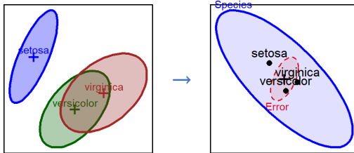
heplot(mod) 2D HE plot for two responses
