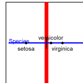
heplot1d(mod) 1D HE plot: H & E as intervals
