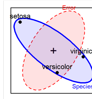
heplot(mod, size = "effect") effect-size scaling: H and E on the data scale
