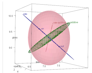
heplot3d(mod) 3D HE ellipsoids (rgl); spin & zoom
