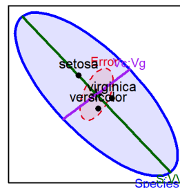
heplot(mod, hypotheses = hyp) 1-df contrasts are drawn as lines : e.g., setosa vs. others; versicolor vs. virginica
