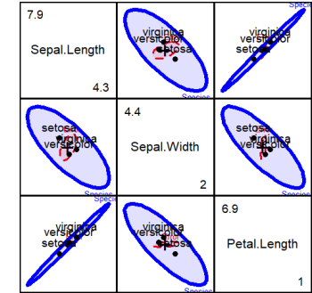
pairs(mod) all pairwise HE plots: an HE plot matrix
