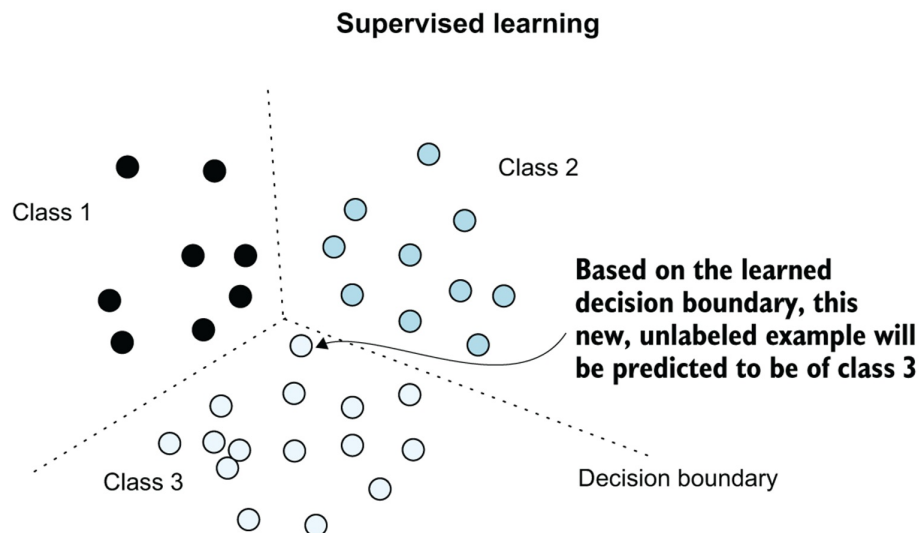
Figure 3.1 A visual representation of supervised classification with a learned decision boundary.
