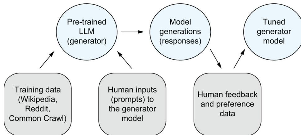
Figure 3.2 The general setup for reinforcement learning with human feedback (RLHF).
