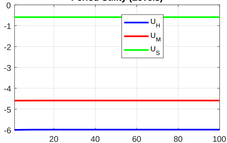
Period Utility (Levels)
