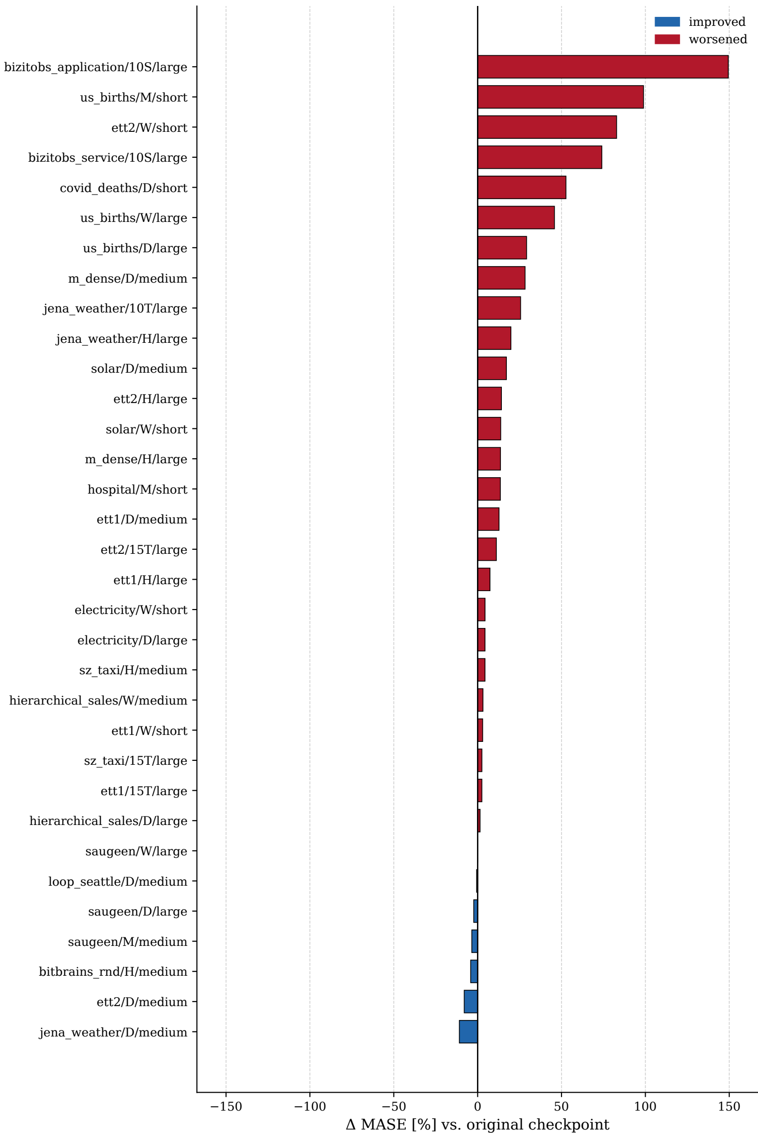
Relative change in MASE - checkpoint 4
