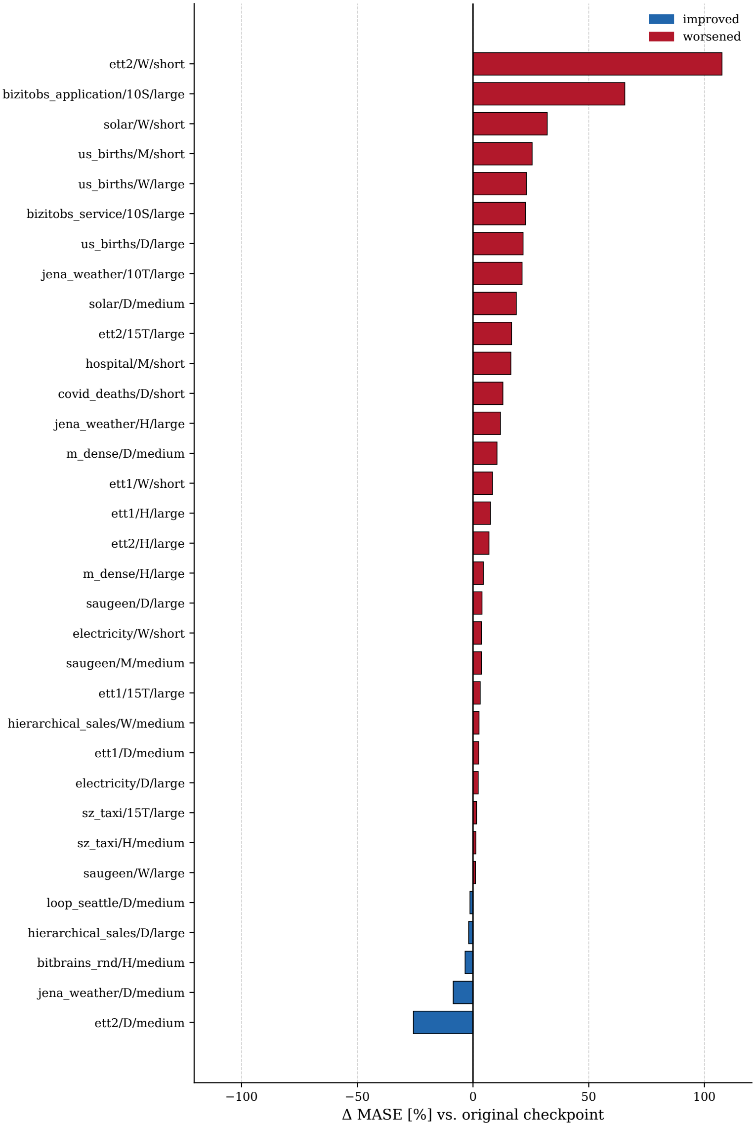
Relative change in MASE - checkpoint 5
