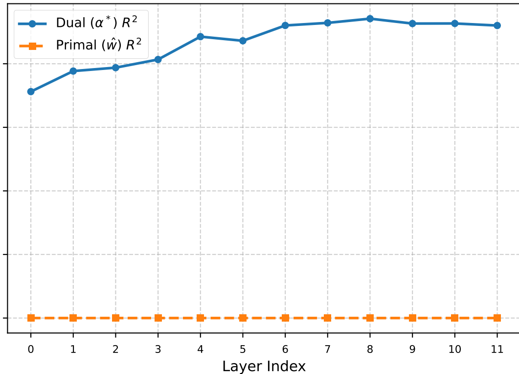
TabICL_v2: Solution Probing R^2
