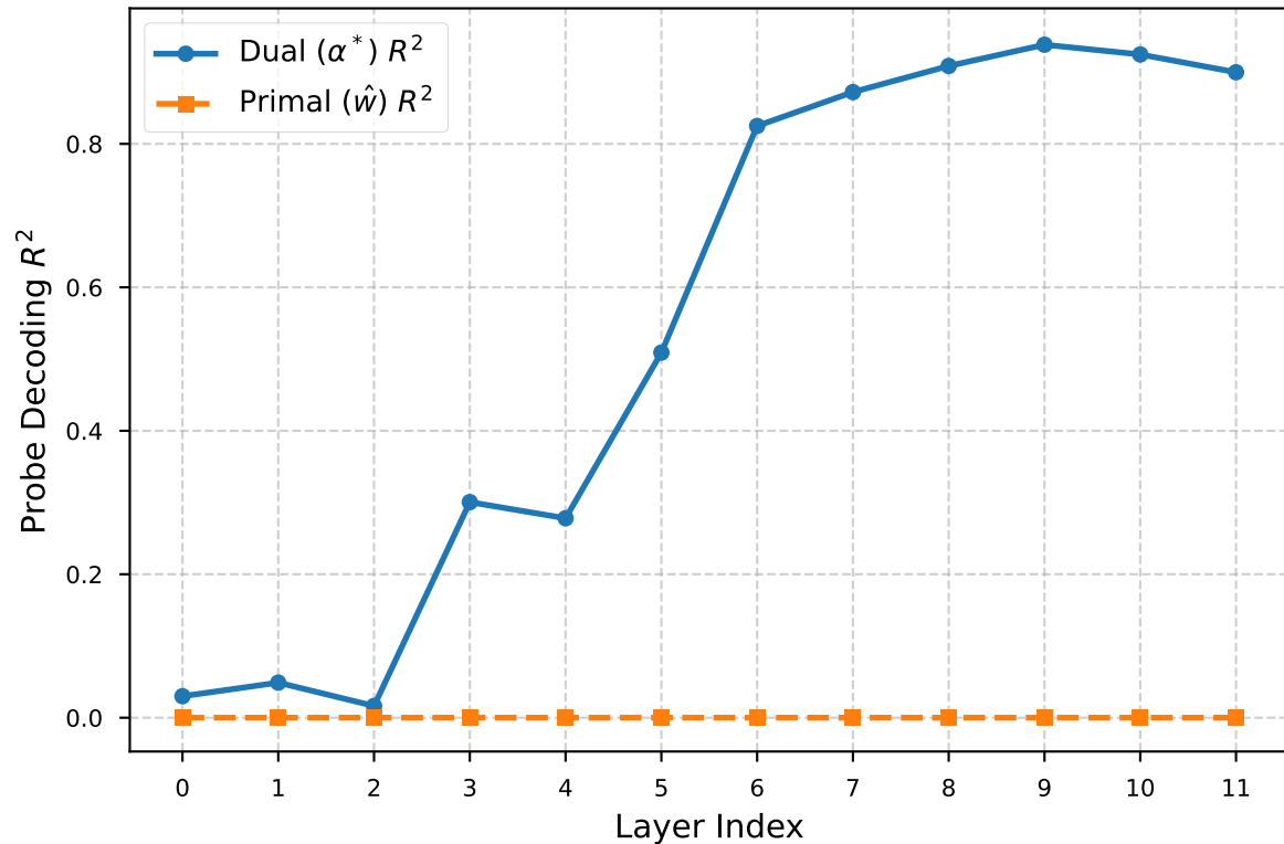
TabPFN_v2: Solution Probing R^2
