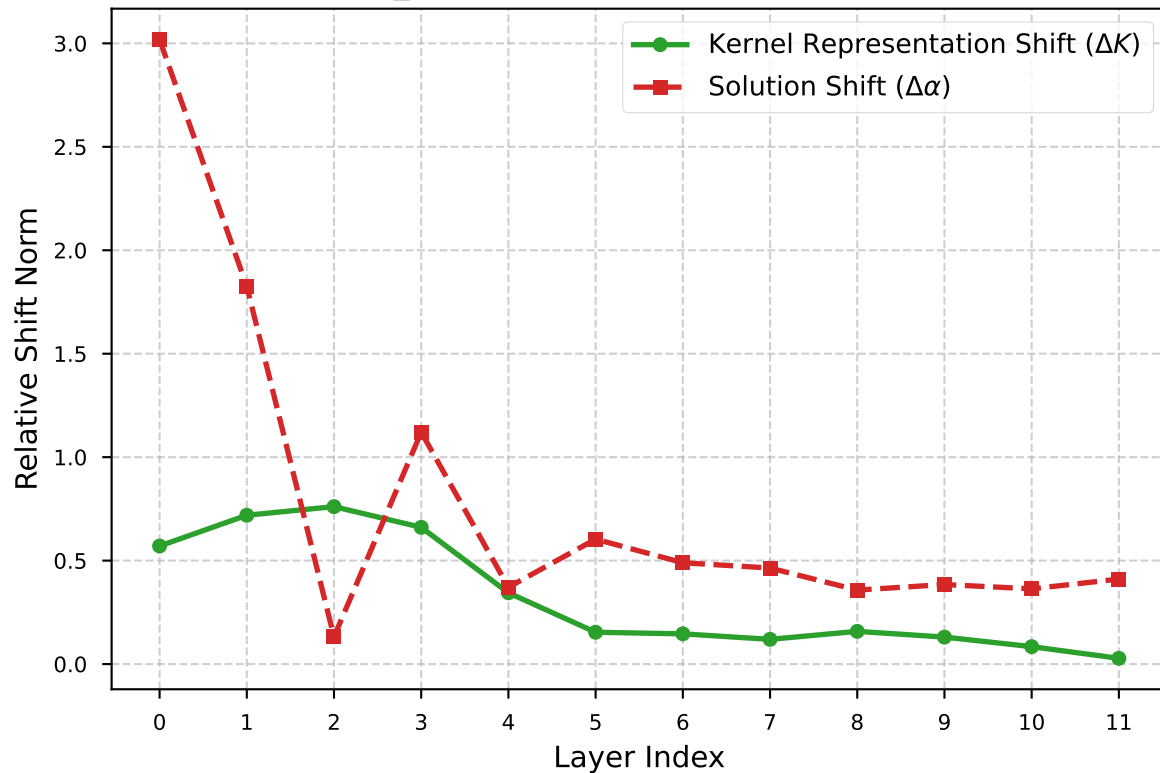
TabPFN_v2: Label Perturbation Sensitivity
