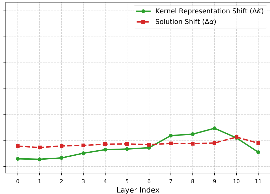
TabICL_v2: Label Perturbation Sensitivity
