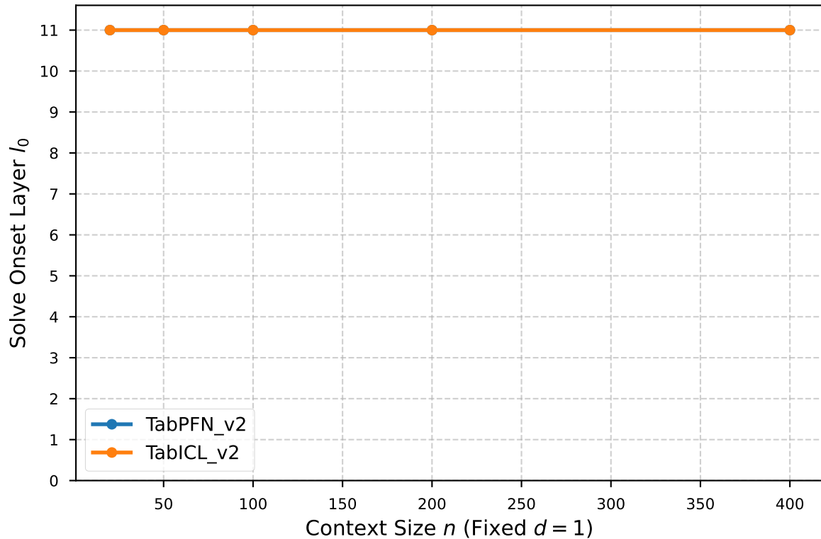
Solve Onset Layer l_0 vs. Context Size n
