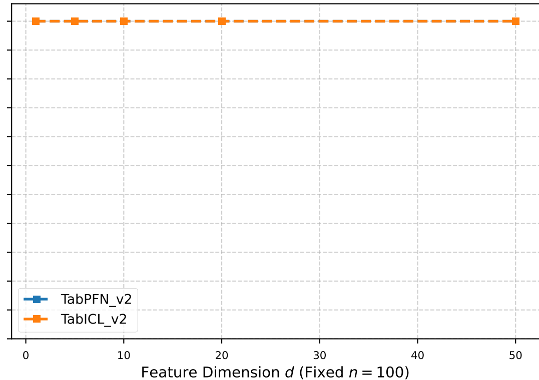
Solve Onset Layer l_0 vs. Feature Dimension d
