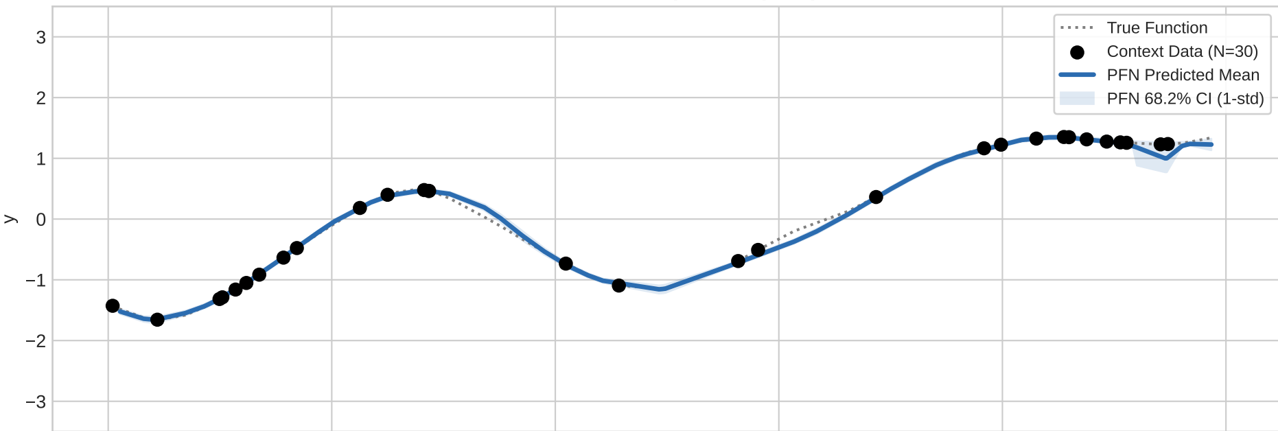
In-Distribution (GP Sample 2)
