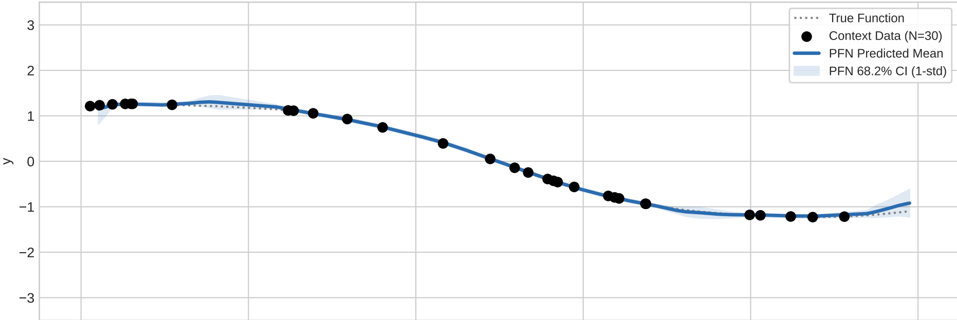
Out-of-Distribution (Periodic Sample 1)
