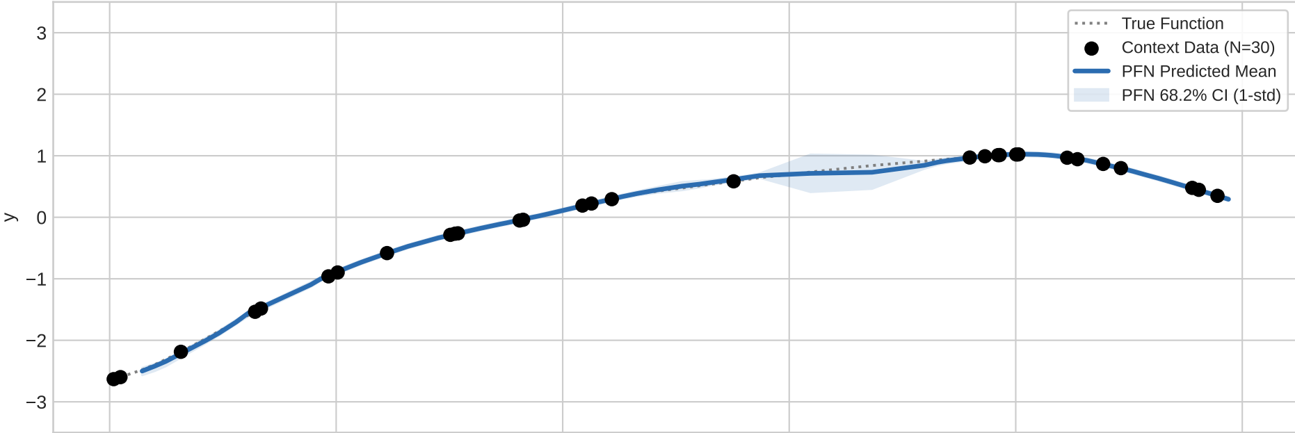
In-Distribution (GP Sample 3)
