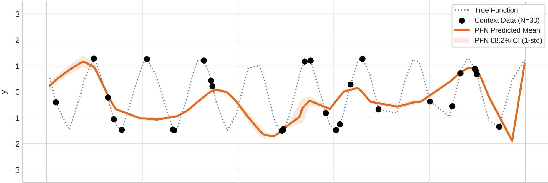
Out-of-Distribution (Periodic Sample 2)
