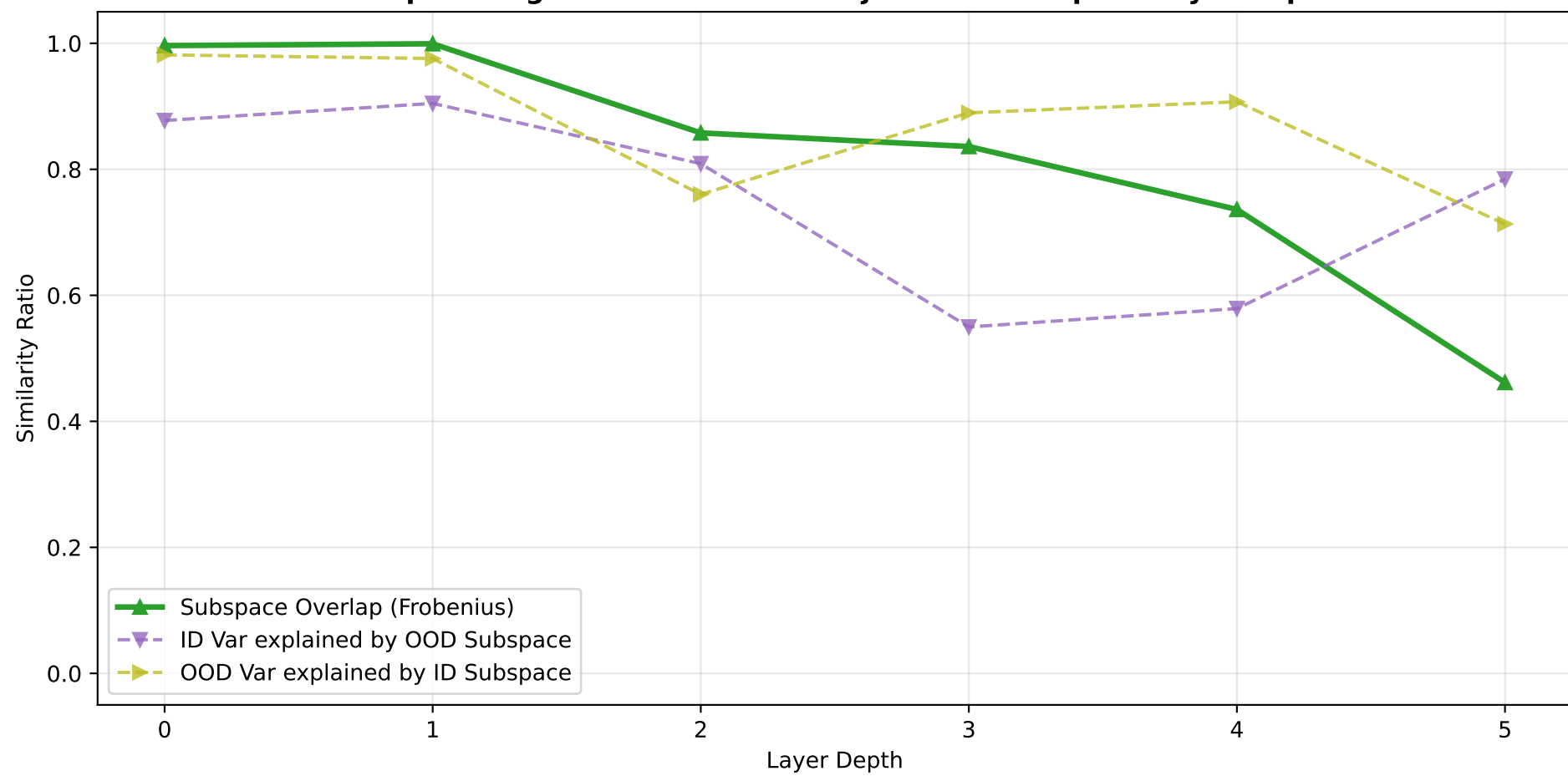
Subspace Alignment and Cross-Projection Overlap vs. Layer Depth
