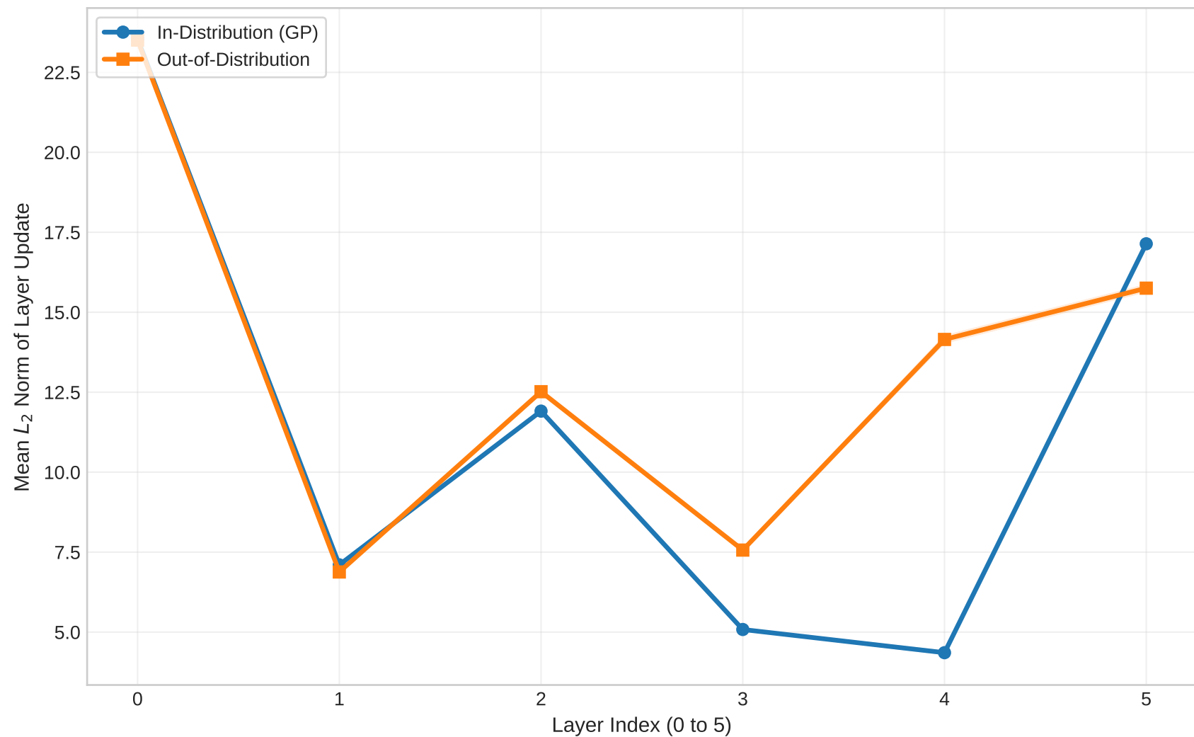
Residual Stream Update Magnitude per Layer (5 Seeds)
