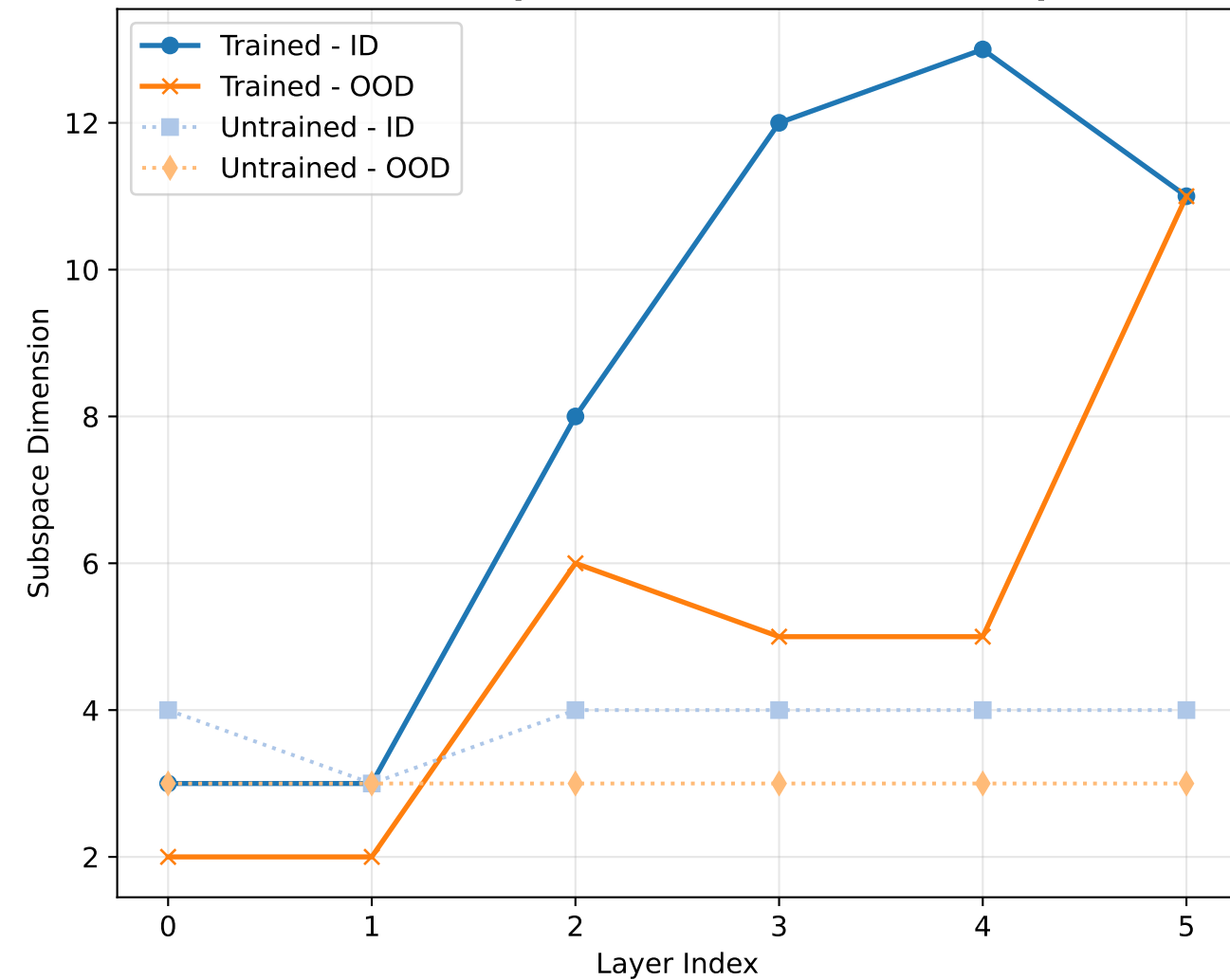
Intrinsic Subspace Dimension ( d_{95} ) vs. Depth
