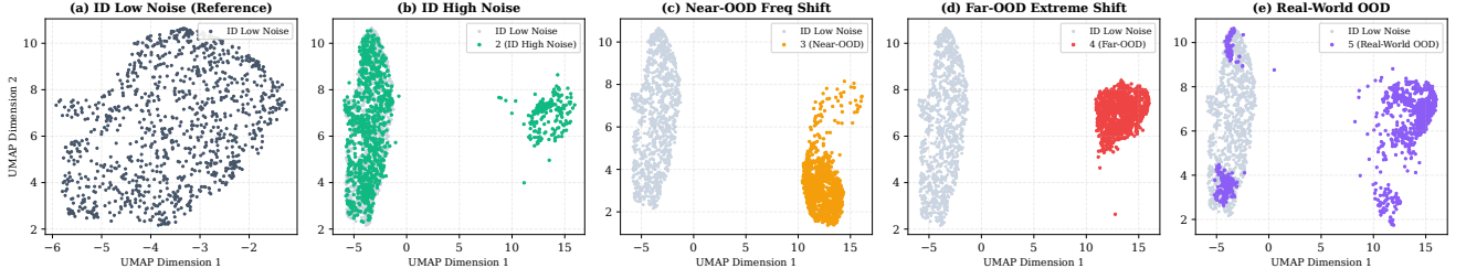
Figure 1: Joint-fitted UMAP projection of Layer 5 activations showing (a) the pure calibration manifold reference set (blue), and (b–e) comparisons against the four evaluation test suites. High observation noise (b) remains overlapping with the calibration manifold, while Near-OOD frequency shift (c), Far-OOD extreme frequency shift (d), and Real-World OOD (e) show distinct topological separation.
