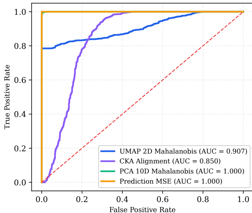
Real-World OOD Detection
