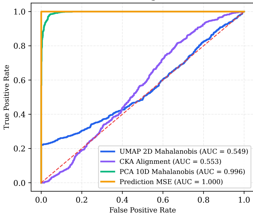
Robustness to Noise (Target: Random Chance)
