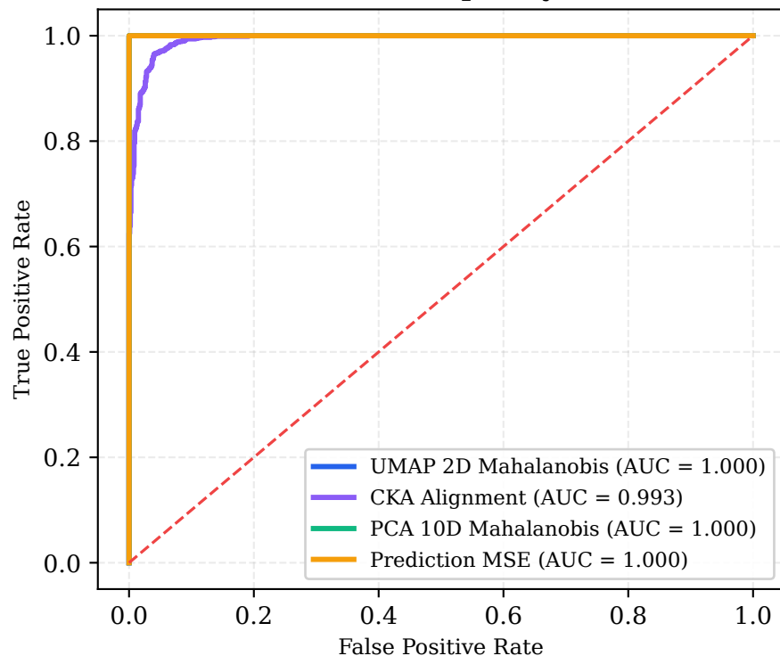
Near-OOD Frequency Shift
