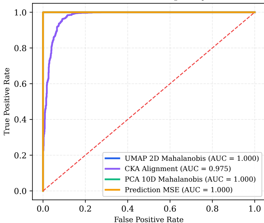
Far-OOD Extreme Frequency Shift
