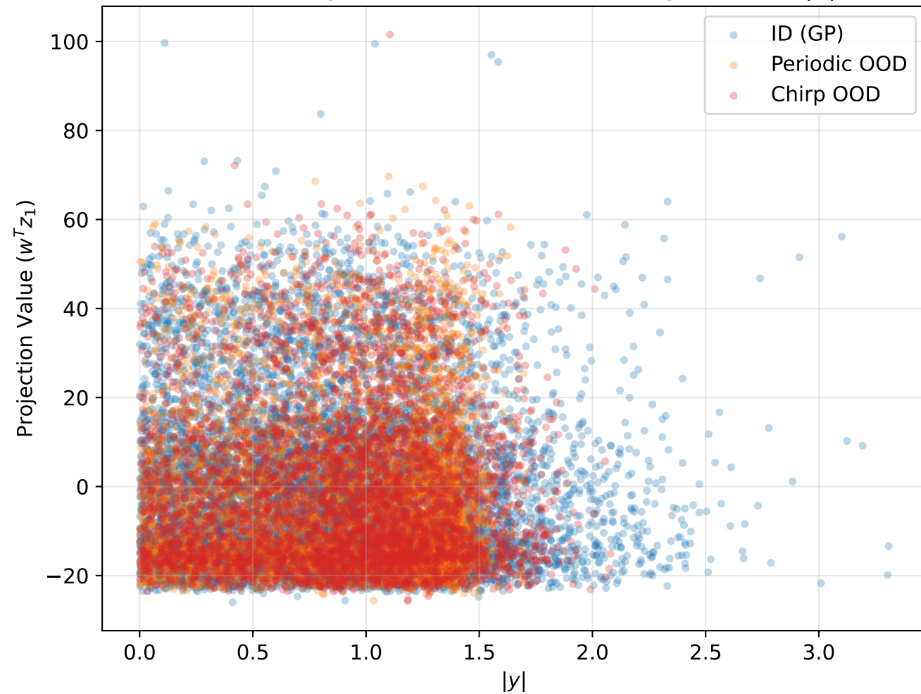
Probe Projection vs. Absolute Target Value |y|
