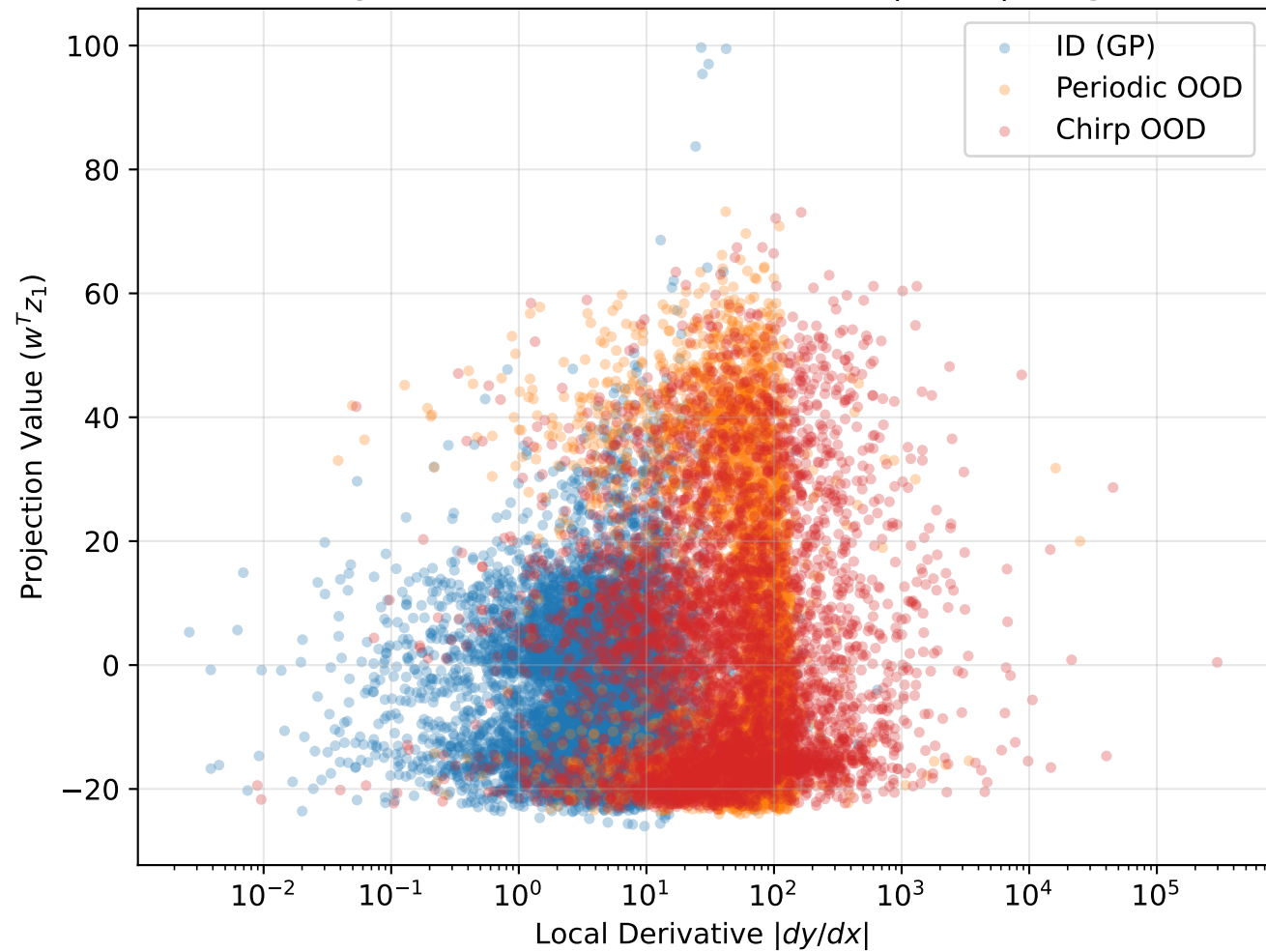
Probe Projection vs. Local Derivative |dy/dx| (Log Scale)
