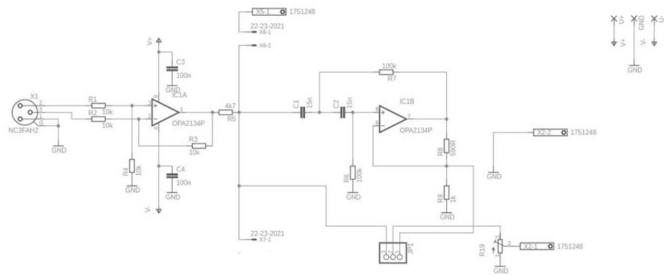
Figure 7 Input Filter Design
