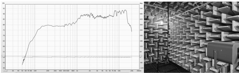
Figure 4 Frequency Response at 0° measured at the anechoic chamber in MDW University Vienna 506x153mm (300 x 300 DPI)
