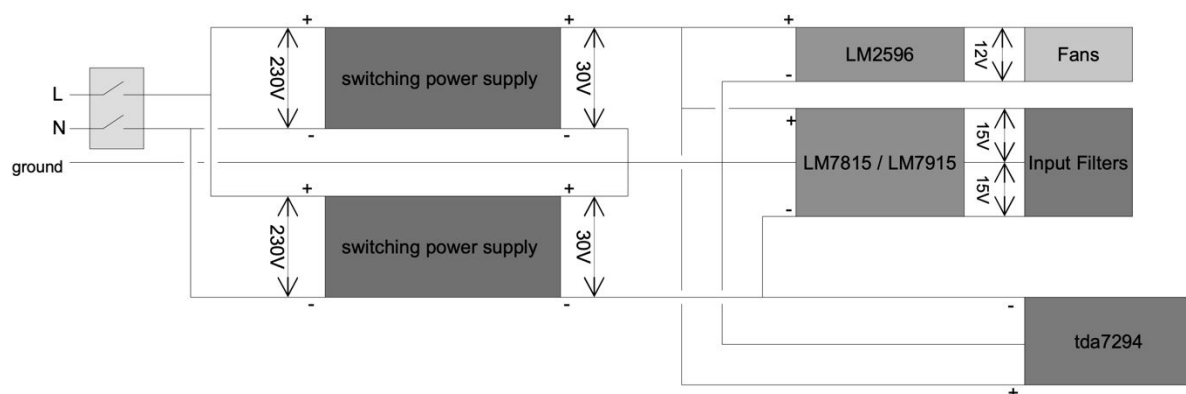
Figure 6 OTTOsonics Power Supply Design
