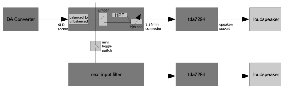
Figure 5 OTTOsonics Amplifier: Design and Signal Flow
