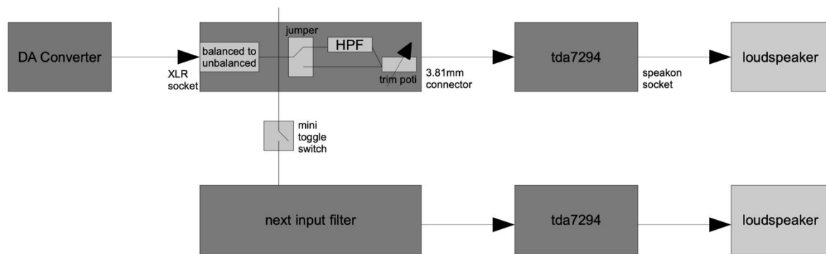
Figure 5 OTTOsonics Amplifier: Design and Signal Flow
