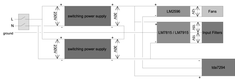
Figure 6 OTTOsonics Power Supply Design 209x75mm (300 x 300 DPI)
