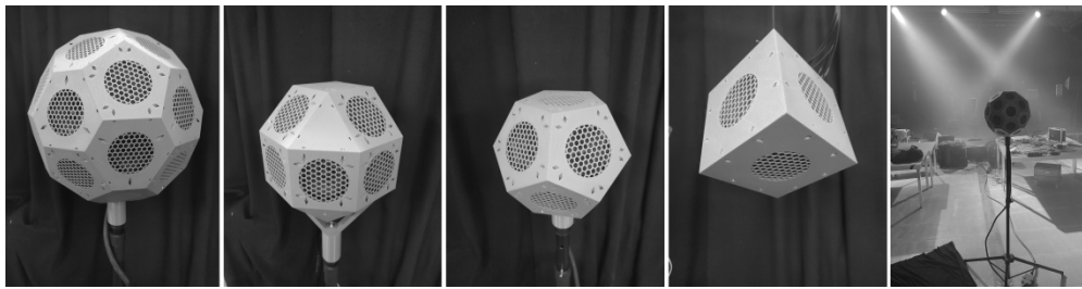
Figure 13 Speaker Arrays created with OTTOsonics with 31, 18, 11 and 6 drivers. Right: setup for performance during Klangfestival 2024
