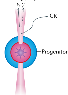
e Engine-driven supernova
