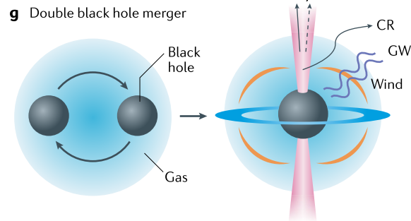
g Double black hole merger
