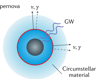
f Supernova
