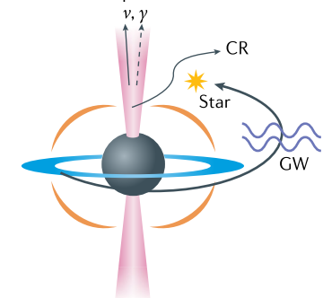
c Tidal disruption event
