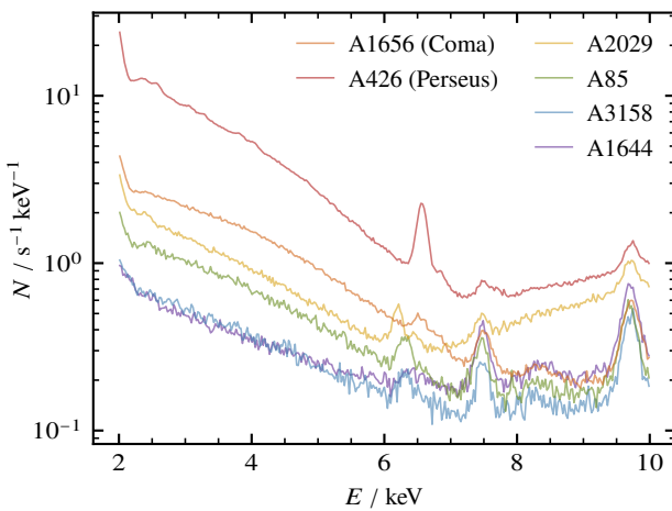
Figure 5: Collection of Chandra binned spectra for various galaxy clusters (Weisskopf et al. 2000). Note the presence of emission lines, as well as possible hints of excesses in the relative count rates for both the soft and hard X-ray regimes.
