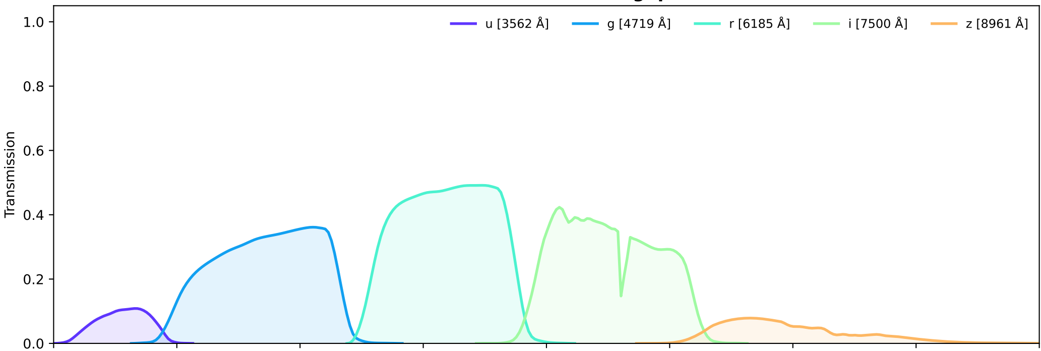
LSST Instrument Throughput
