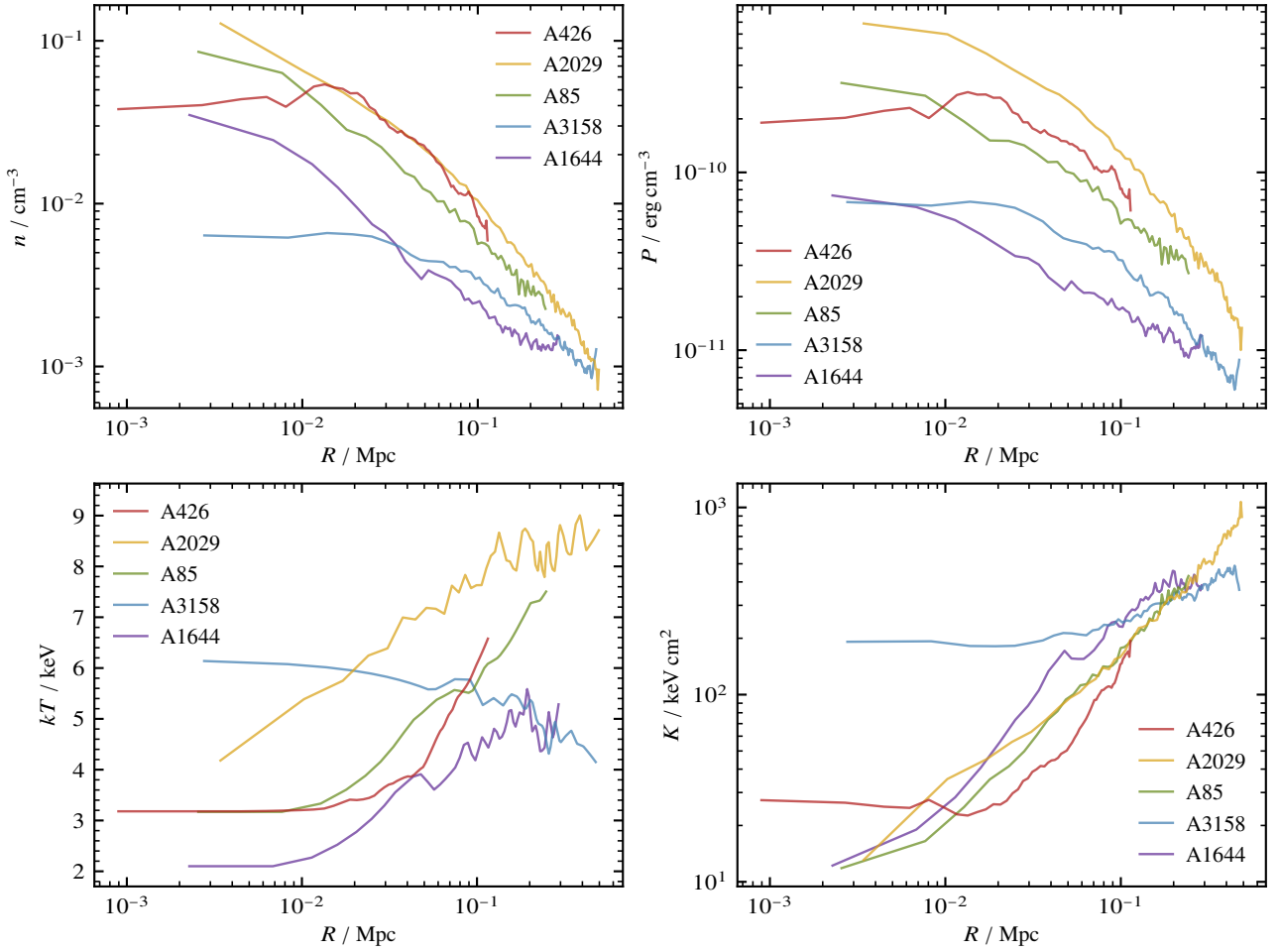
Figure 7: Sample of galaxy cluster radial profiles from Chandra observations (Weisskopf et al. 2000, Cavagnolo et al. 2009). Top Left: Electron number density. Top Right: Gas pressure. Bottom Left: Gas temperature. Bottom Right: Gas entropy. Compare to Figure 6 for a visualization of theoretical and empirical fits with realistic parameter choices.
