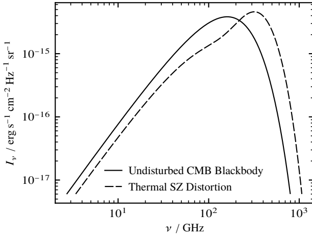
Figure 5: Schematic view of the Sunyaev-Zel'dovich effect with exaggerated Y = 0.175 Compton factor.
