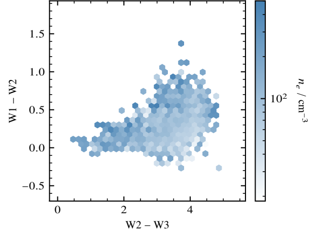
Figure 19: Binned WISE data showing electron density.
