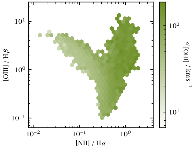
Figure 13: Binned BPT data showing gas velocity. Refer to Figures 20 and 21 for WHAN and WISE plots.
