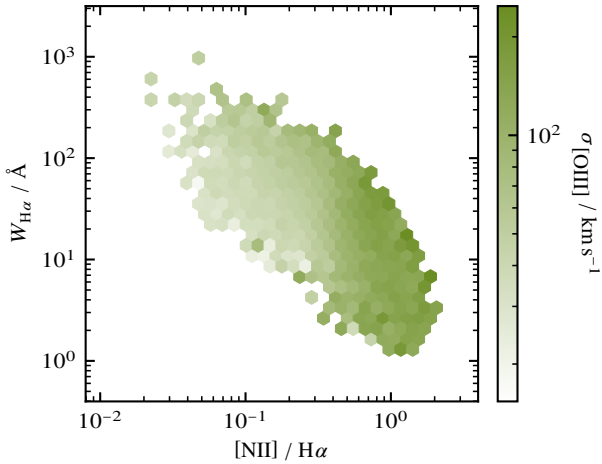
Figure 20: Binned WHAN data showing gas velocity.
