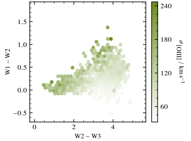
Figure 21: Binned WISE data showing gas velocity.
