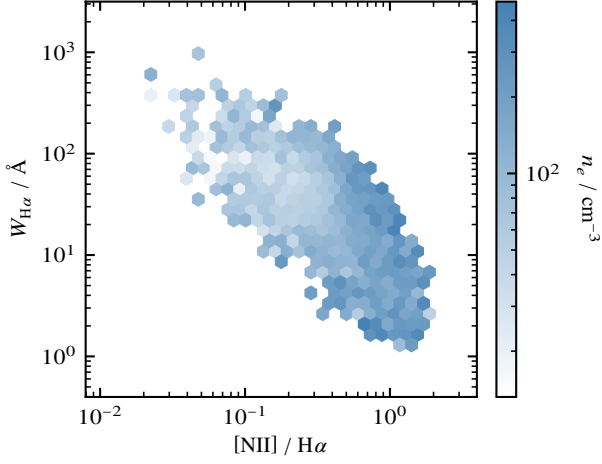
Figure 18: Binned WHAN data showing electron density.
