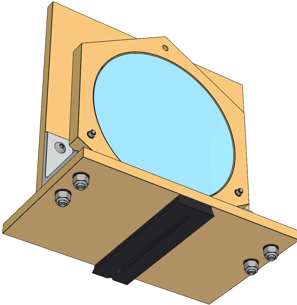
Fig. 12. Mirror cell from below: the quick-release sliding plate on the underside of the base, and the bracket locknuts
