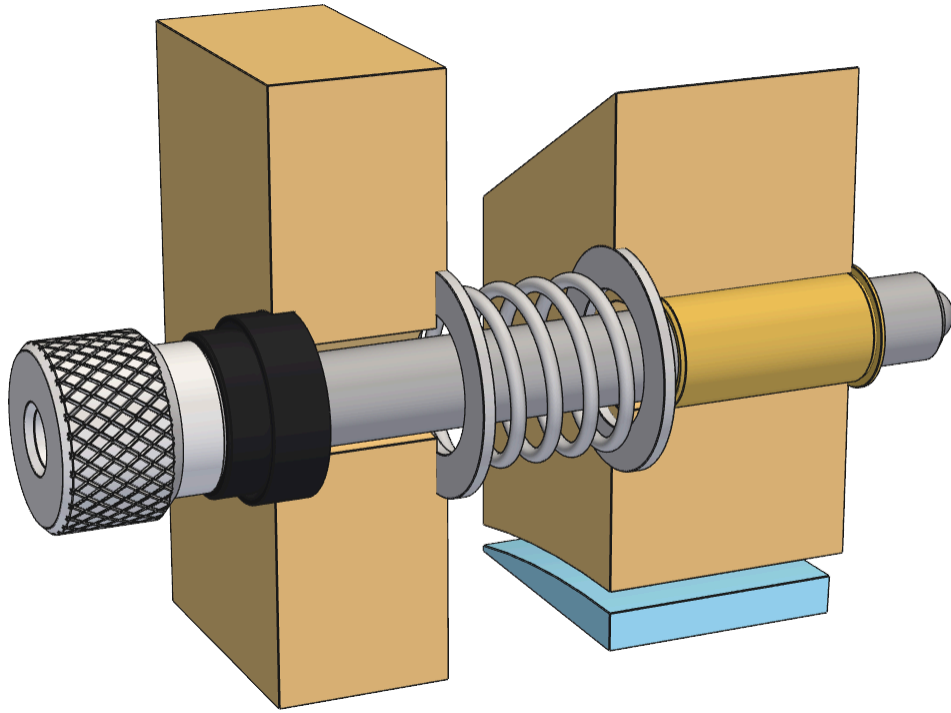
Fig. 11. Adjuster station, plywood and mirror cut away: knob, spherical washer pair, spring and seat washers, bushing, and adjuster screw
