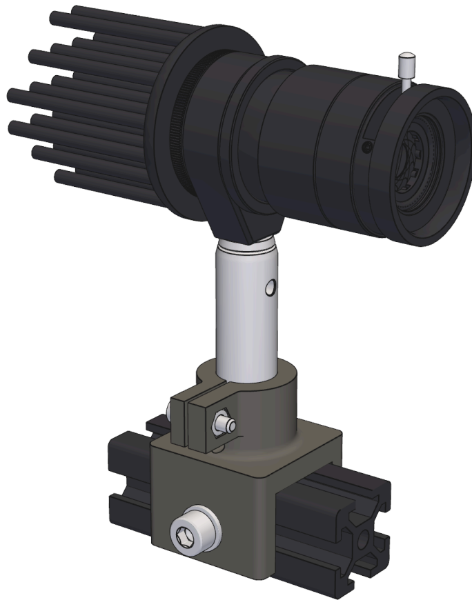
Fig. 4. Light source on rail: heatsink and LED module, SMR1/M, SM1V05, SM1L03, and iris
