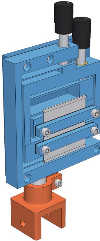
Fig. 7. Flexure slit head on its post and rail shoe, seen from the light-source side: blades and clamp bars, FAS100 centering and width adjusters
