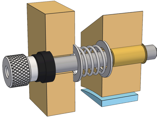
Fig. 12. Adjuster station, plywood and mirror cut away: knob, spherical washer pair, spring and seat washers, bushing, and adjuster screw
