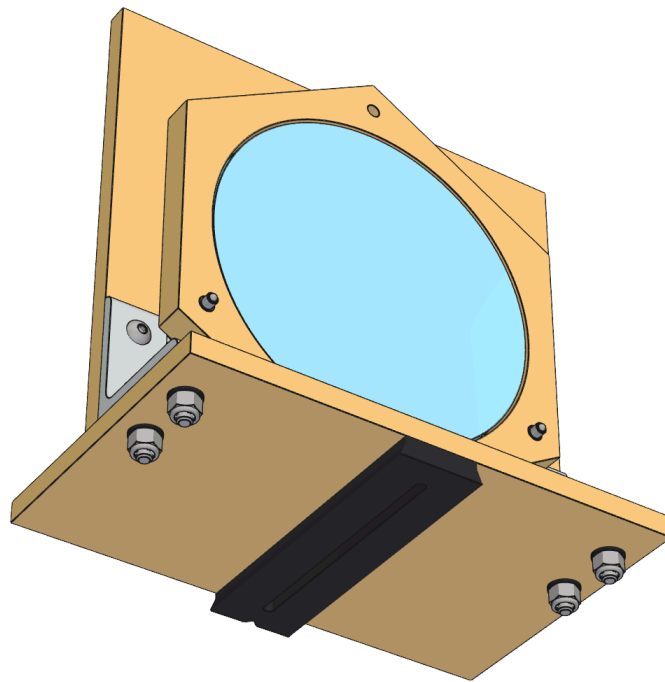
Fig. 13. Mirror cell from below: the quick-release sliding plate on the underside of the base, and the bracket locknuts
