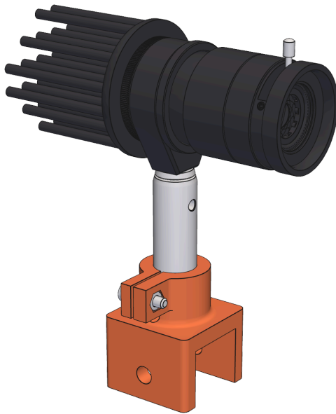
Fig. 4. Light source on its post and rail shoe: heatsink and LED module, SMR1/M, SM1V05, SM1L03, and iris
