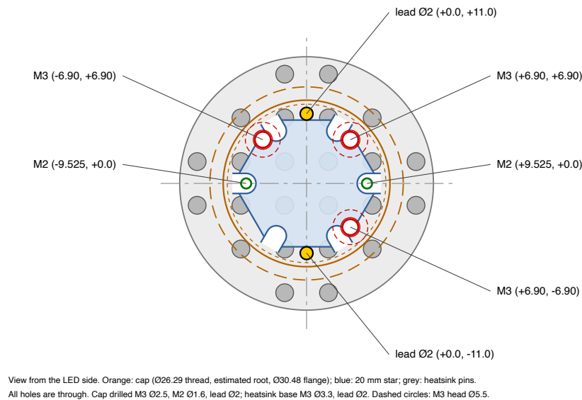
Fig. 6. Cap and heatsink hole layout, seen from the LED side, in the frame of the heatsink pin lattice
