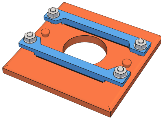
Fig. 9. Cassette blank with its two clamp bars and hardware
