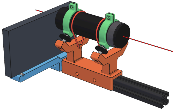
Fig. 10. Lens cradle and phone rest on the imaging rail, with phone and lens envelopes
