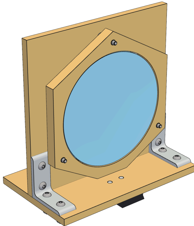
Fig. 11. Mirror cell from the mirror side: base plate, cell-adjuster plate, moving mirror plate and mirror, and corner brackets
