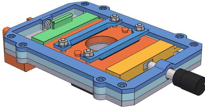
Fig. 8. Cutoff carriage with a seated cassette: guide frame, keeper plate, driven and spring plungers, and the FAS100 fine adjuster
