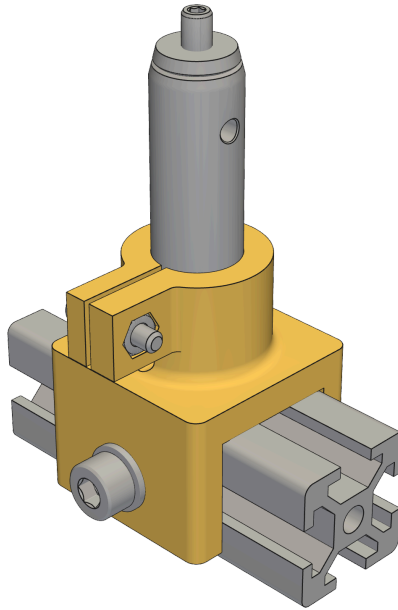
Fig. 3. Common rail shoe on rail with TR50/M post
