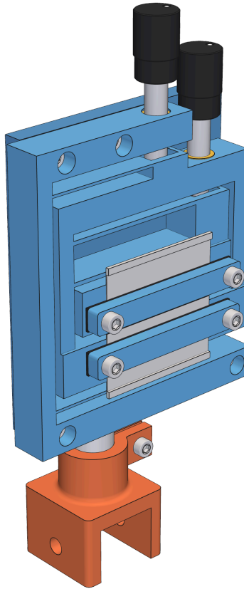
Fig. 7. Flexure slit head on its post and rail shoe, seen from the light-source side: blades and clamp bars, FAS100 centering and width adjusters
