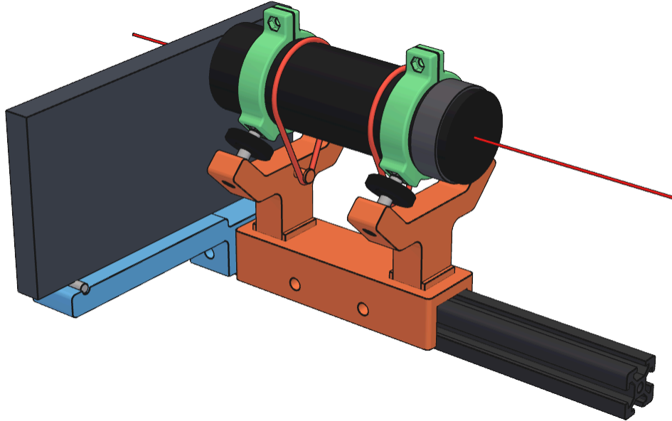
Fig. 6. Lens pointer and phone rest on the imaging rail, with phone and lens envelopes
