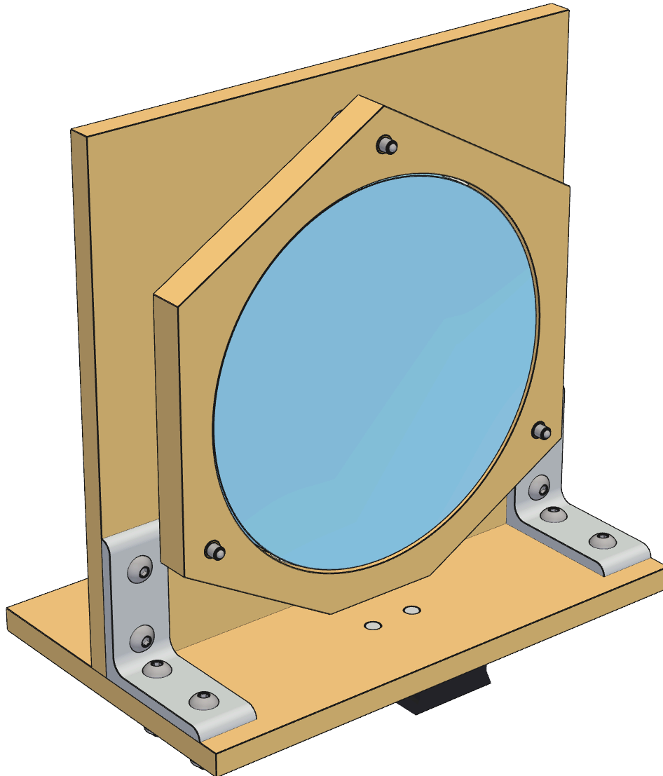
Fig. 10. Mirror cell from the mirror side: base plate, cell-adjuster plate, moving mirror plate and mirror, and corner brackets
