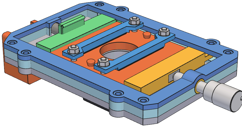
Fig. 7. Cutoff carriage with a seated cassette: guide frame, keeper plate, driven and spring plungers, and the FAS100 fine adjuster
