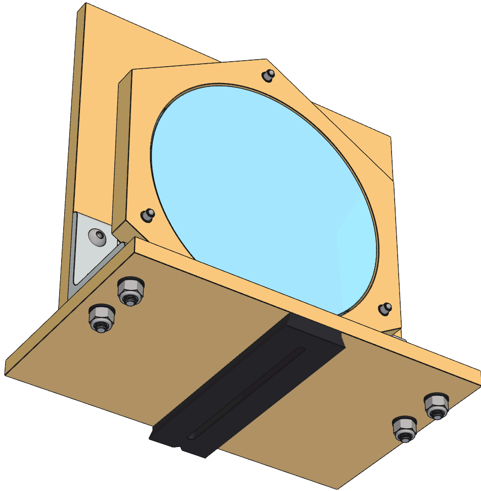
Fig. 12. Mirror cell from below: the quick-release sliding plate on the underside of the base, and the bracket locknuts
