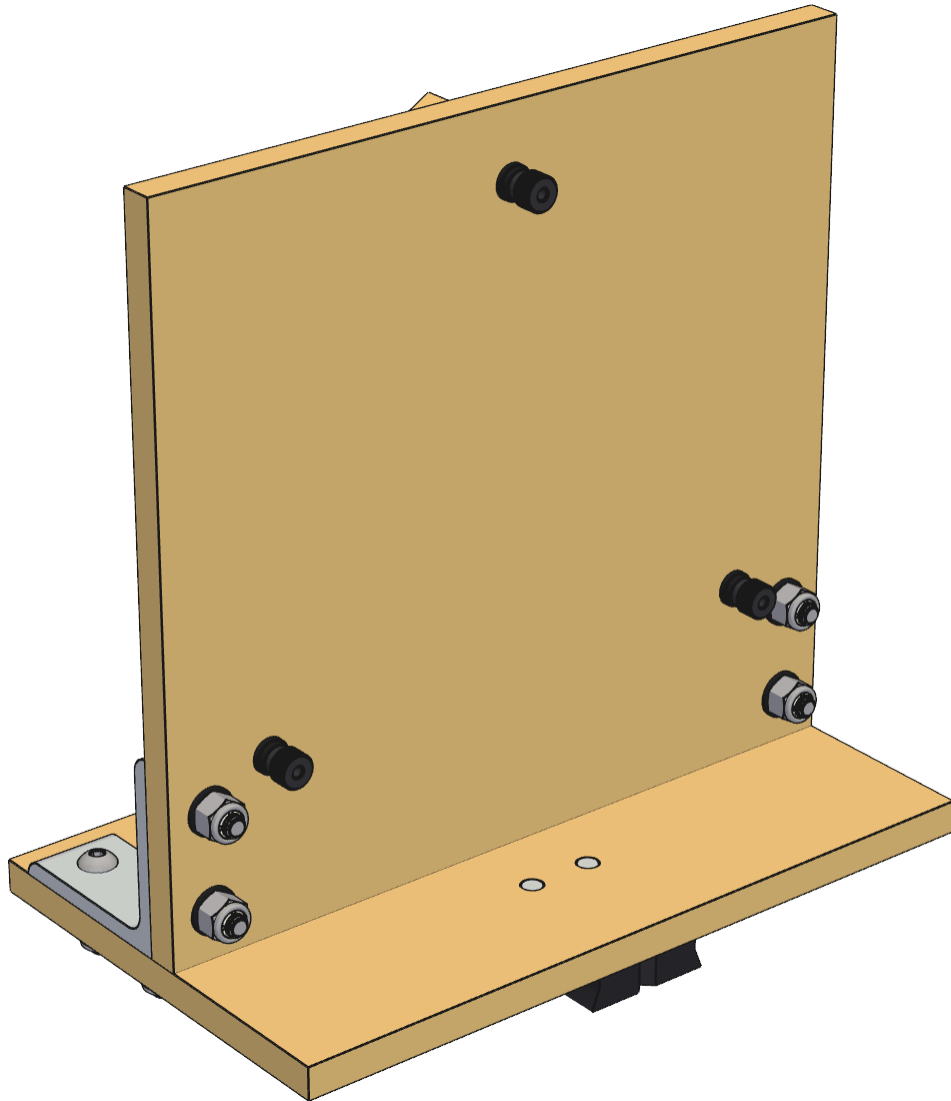
Fig. 11. Mirror cell from behind: the three adjuster knobs on their spherical washers, and the bracket washers and locknuts
