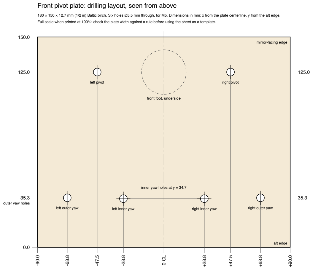
Fig. 2. Front pivot plate drilling layout, seen from above, in plate coordinates
