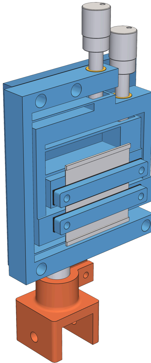
Fig. 6. Flexure slit head on its post and rail shoe, seen from the light-source side: blades and clamp bars, FAS100 centering and width adjusters
