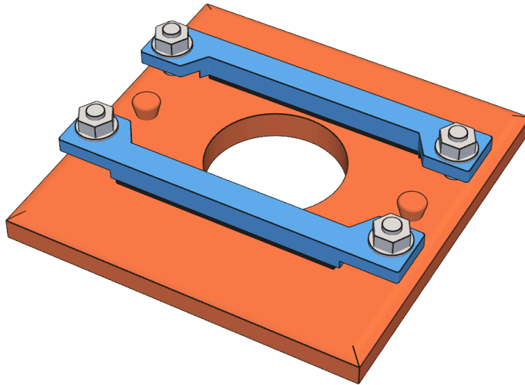
Fig. 8. Cassette blank with its two clamp bars and hardware
