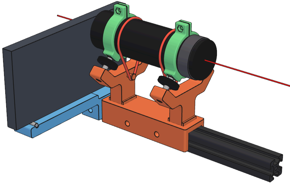
Fig. 9. Lens pointer and phone rest on the imaging rail, with phone and lens envelopes
