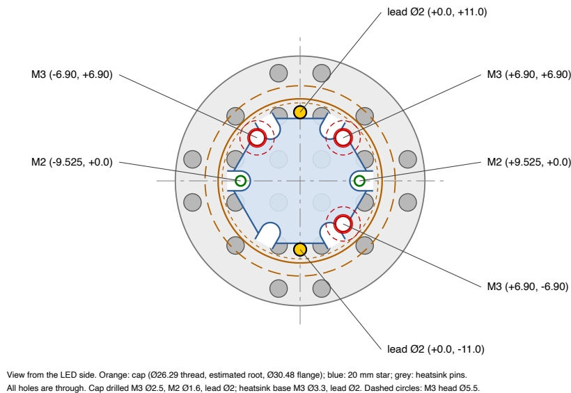
Fig. 5. Cap and heatsink hole layout, seen from the LED side, in the frame of the heatsink pin lattice
