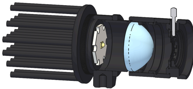
Fig. 5. Light source cutaway
