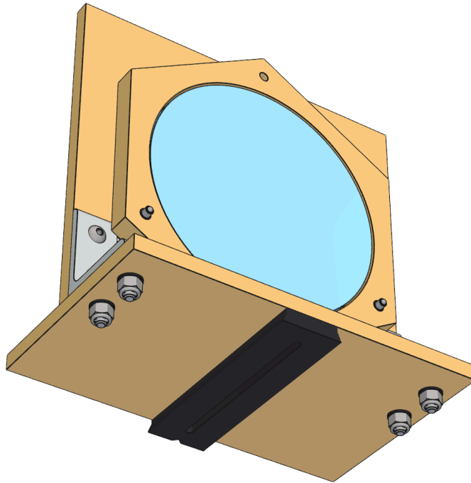
Fig. 13. Mirror cell from below: the quick-release sliding plate on the underside of the base, and the bracket locknuts
