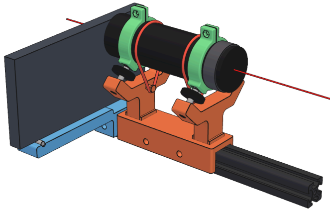
Fig. 10. Lens pointer and phone rest on the imaging rail, with phone and lens envelopes
