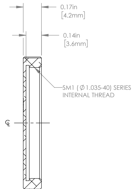
SECTION X-X
