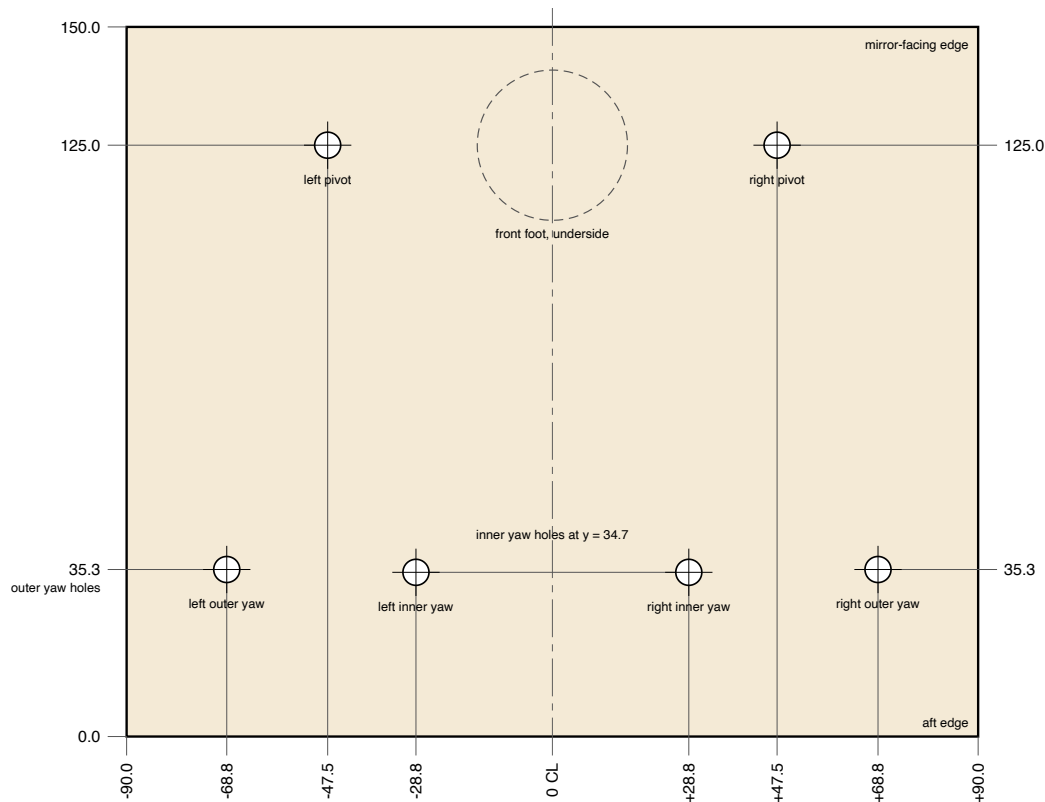
Fig. 2. Front pivot plate drilling layout, seen from above, in plate coordinates
