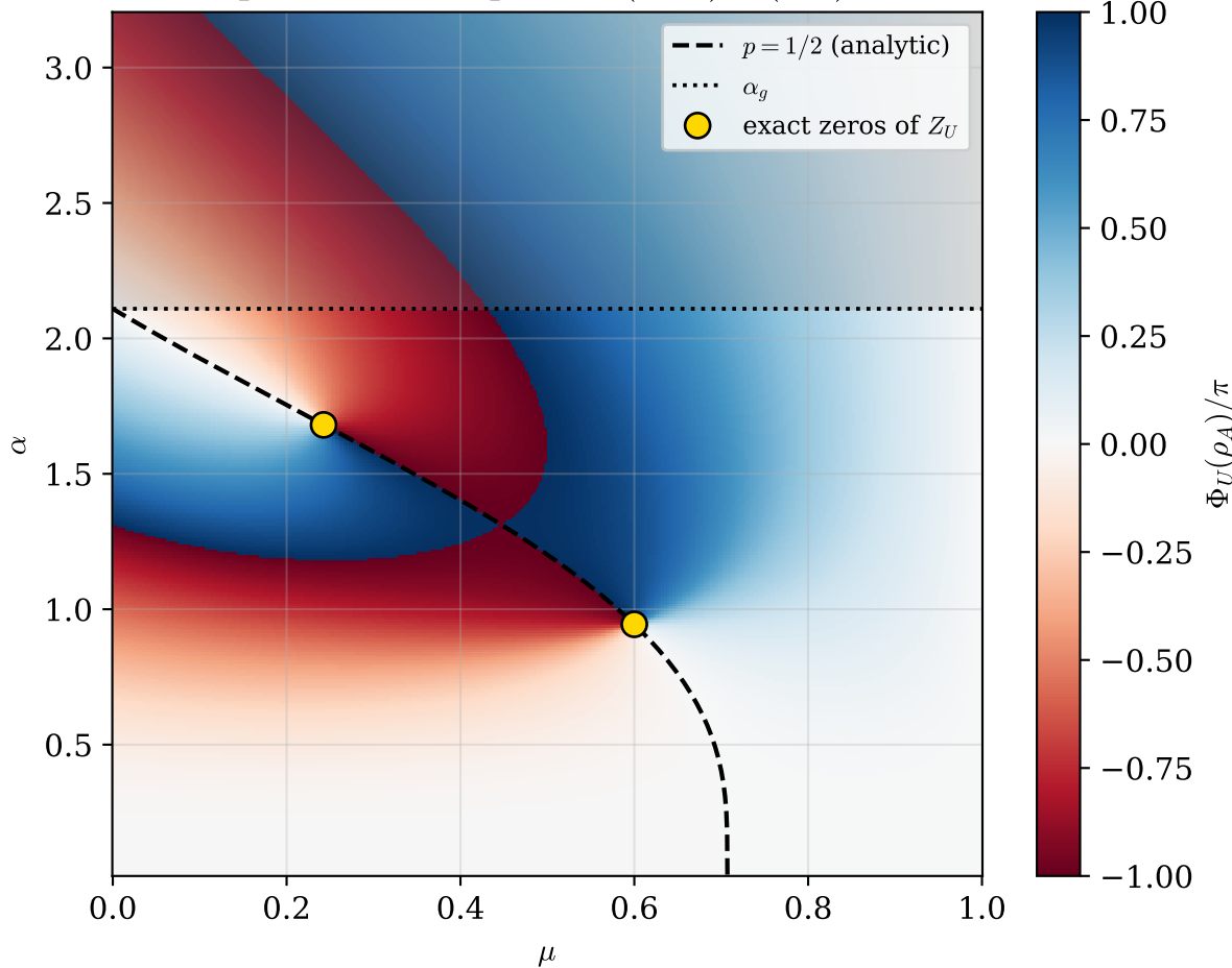
Principal Uhlmann phase, (m, n) = (0, 2) , \Delta = 2
