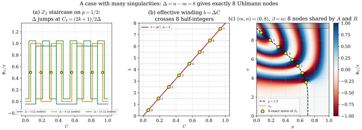
Figure 15: A case with many singularities, \Delta = n - m = 8 . (a) The \mathbb{Z}_2 staircase of Eq. (40) now takes \Delta steps; curves for \Delta = 4, 8, 12 are offset vertically. (b) The effective winding b = \Delta C crosses \Delta = 8 half-integers, one per node (gold, labelled by k ). (c) The eight nodes in the (\mu, \alpha) plane for the symmetric family \beta = \alpha , strung along the p = 1/2 curve and all below \alpha_g = 9.23 ; since p_A = p_B there, these eight points are the nodes of both subsystems.
