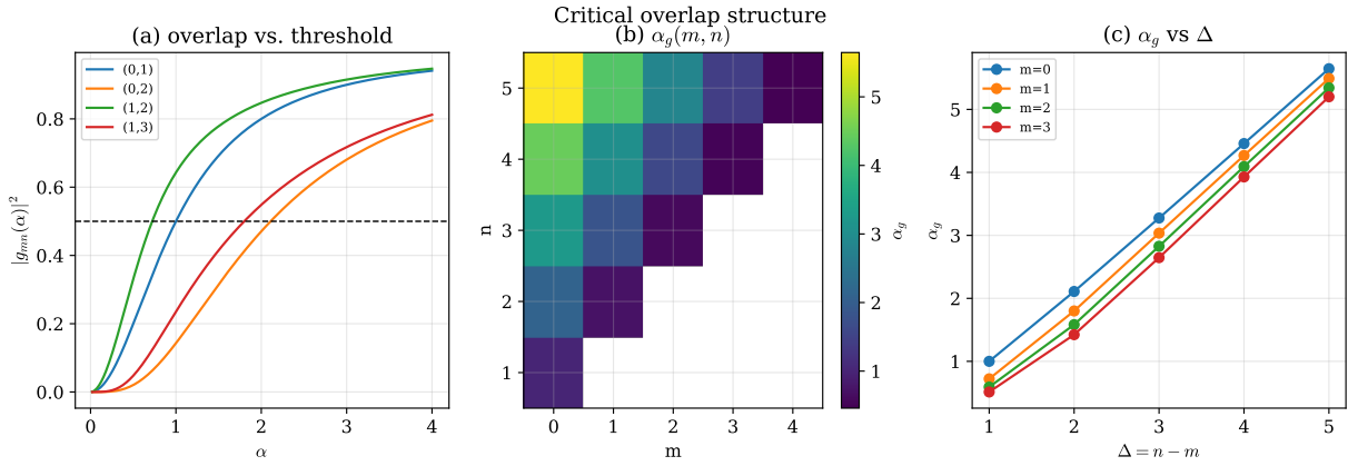
Figure 9: Critical overlap structure. (a) |g_{mn}(\alpha)|^2 against the threshold 1/2 . (b) The discrete critical function \alpha_g(m, n) over the grid of Table 3. (c) \alpha_g versus \Delta for several fixed m : larger photon-addition separation extends the nodal region to larger coherent amplitude.
