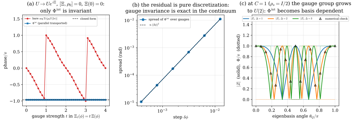
Figure 19: Gauge invariance of the interferometric phase, Sec. 12.2. (a) Under the one-parameter gauge family U \rightarrow U e^{it\Xi(\phi)} with [\Xi, \rho_0] = 0 and \Xi(0) = 0 , the bare Pancharatnam phase \text{Arg Tr}[\rho_0 U(2\pi)] sweeps the entire circle while \Phi^{\text{int}} stays pinned to the closed form (62) (dashed). (b) The residual spread of \Phi^{\text{int}} over gauges scales as (\delta\phi)^2 : gauge invariance is exact in the continuum and the residual is purely the discretization of the transport integral. (c) At C = 1 , where \rho_s = I/2 and the gauge group grows to U(2) , the phase becomes basis dependent: |Z^{\text{int}}| = |\cos(\pi\Delta \cos \theta_Q)| as a function of the eigenbasis angle, Eq. (68), with zeros whenever \Delta \cos \theta_Q is a half-integer (triangles: direct numerical evaluation of Eq. (53)).
