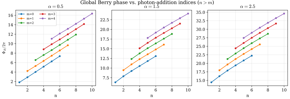
Figure 2: Discrete dependence of the global Berry phase on the photon-addition indices at three coherent amplitudes. Only n > m is shown, the ordering in which the overlap formula (72) is written.
