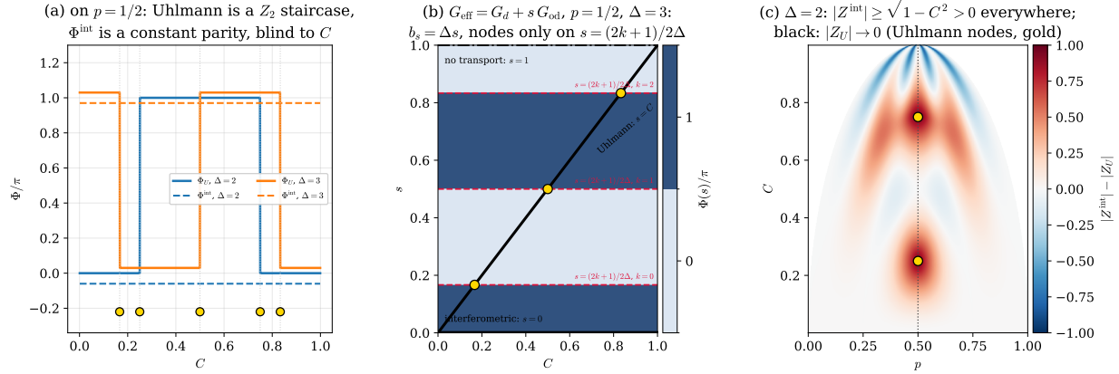
Figure 18: The two mixed-state geometric phases on the same logical loop, Eq. (63). (a) On p = 1/2 : the Uhlmann phase is the \mathbb{Z}_2 staircase of Eq. (40), jumping at the quantized concurrences C_k = (2k + 1)/2\Delta (gold), while the interferometric phase is the constant parity \pi\Delta of Eq. (67), blind to C (curves offset vertically for legibility). (b) The interpolating family G_{\text{eff}} = G_d + s G_{od} of Eq. (64) at p = 1/2 , \Delta = 3 : since b_s = \Delta s , all nodes lie on the horizontal lines s = (2k + 1)/2\Delta (dashed). The Uhlmann phase runs along the diagonal s = C and meets every one of them; the interferometric phase runs along s = 0 and meets none; s = 1 is the untransported cycle. (c) Difference of moduli over the physical region (p, C) for \Delta = 2 : |Z^{\text{int}}| \geq \sqrt{1 - C^2} > 0 everywhere, whereas |Z_U| vanishes at the two gold nodes on p = 1/2 (black contour |Z_U| = 0.02 ).
