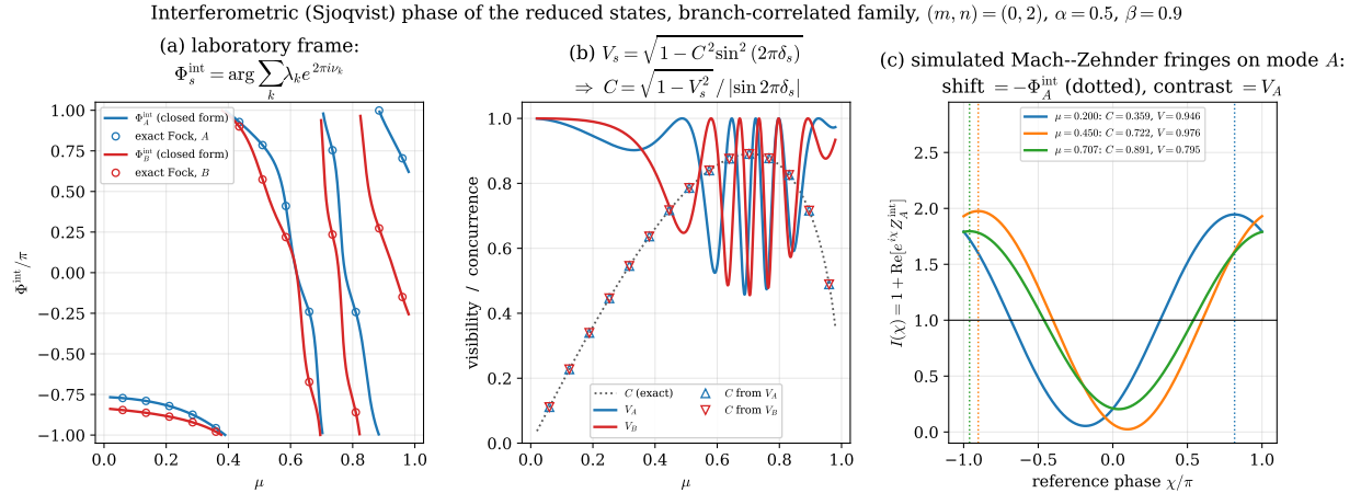
Figure 17: Interferometric (Sjöqvist) phase of the two reduced states in the laboratory frame, Eqs. (56)–(57), for the branch-correlated family with (m, n) = (0, 2) , \alpha = 0.5 , \beta = 0.9 . (a) \Phi_A^{\text{int}} and \Phi_B^{\text{int}} versus \mu : lines are the closed form, markers the exact truncated-Fock evaluation of \text{Arg} \sum_k \lambda_k e^{2\pi i \nu_k} (agreement 4 \times 10^{-14} ). The two subsystems differ because the offsets \pi \text{Tr} \mathcal{N}_s and the splittings \delta_s are local properties of each mode. (b) Fringe contrast \mathcal{V}_s = \sqrt{1 - C^2 \sin^2 2\pi \delta_s} (solid) against the exact concurrence (dotted); triangles are the concurrence reconstructed from the contrast of a single mode through the witness (61), and fall on the exact curve. (c) Simulated Mach-Zehnder fringes I(\chi) = 1 + \text{Re}[e^{i\chi} Z_A^{\text{int}}] at three values of \mu : the fringe shift is -\Phi_A^{\text{int}} (dotted verticals) and the contrast is \mathcal{V}_A .
