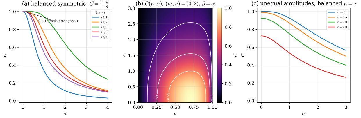
Figure 12: Concurrence of the entangled PACS, Eq. (19). (a) Balanced symmetric family: C = (1 - q)/(1 + q) decreases monotonically from 1 at \alpha \rightarrow 0 (where the PACS reduce to orthogonal Fock states) towards 0 at large \alpha (parallel branches). Larger \Delta keeps the branches distinguishable longer. (b) C over the (\mu, \alpha) plane with contours. (c) Unequal amplitudes: fixing \beta caps the attainable concurrence, since C carries the factor \sqrt{(1 - g_\alpha^2)(1 - h_\beta^2)} .
