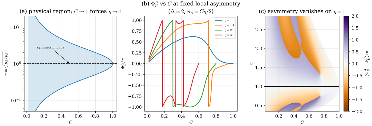
Figure 14: Concurrence and local asymmetry as independent coordinates, Eqs. (35)–(36). (a) The physical region (37) in the (C, \eta) plane; it is symmetric under \eta \rightarrow 1/\eta and pinches to the single point \eta = 1 as C \rightarrow 1 , so maximal entanglement enforces A \leftrightarrow B symmetry. (b) \Phi_U^A versus C at fixed local asymmetry \eta . (c) \Phi_U^A - \Phi_U^B over the same plane: the asymmetry vanishes identically on the line \eta = 1 .
