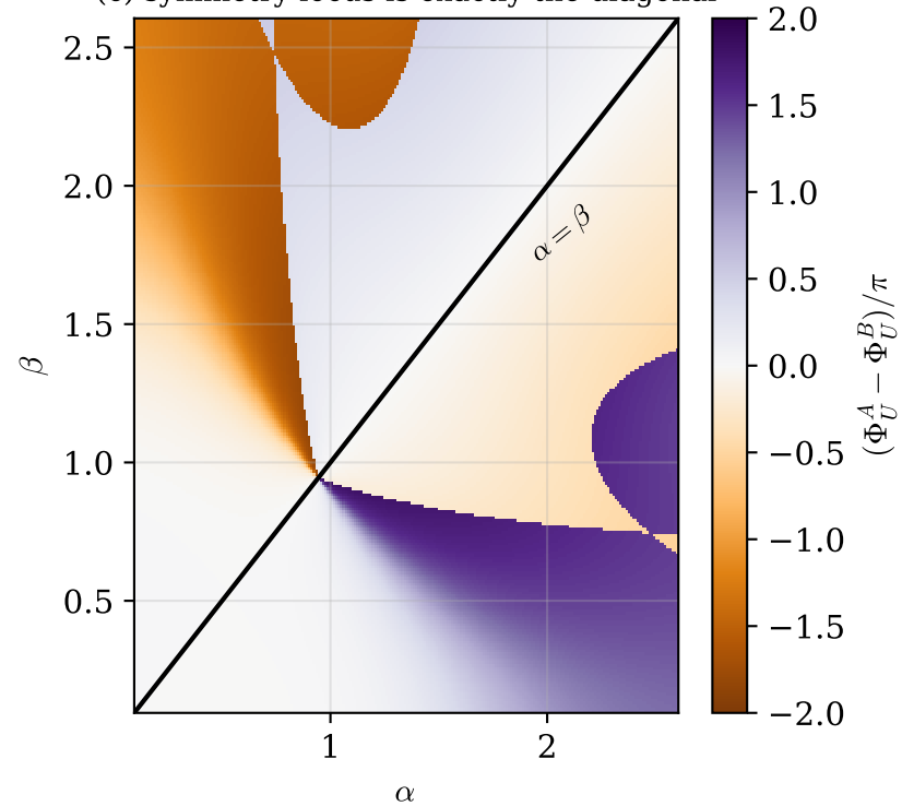
(c) symmetry locus is exactly the diagonal
