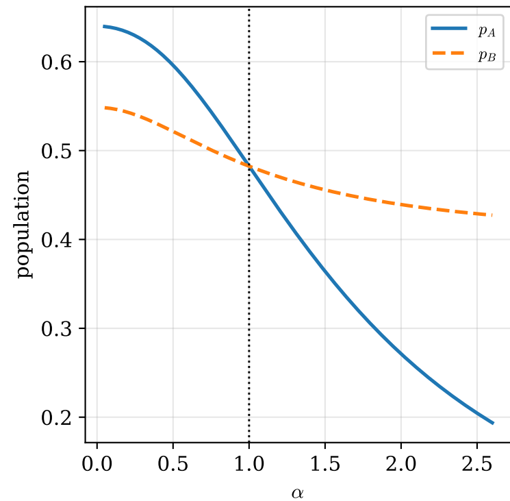
(a) p_A \neq p_B unless \alpha = \beta = 1.0
