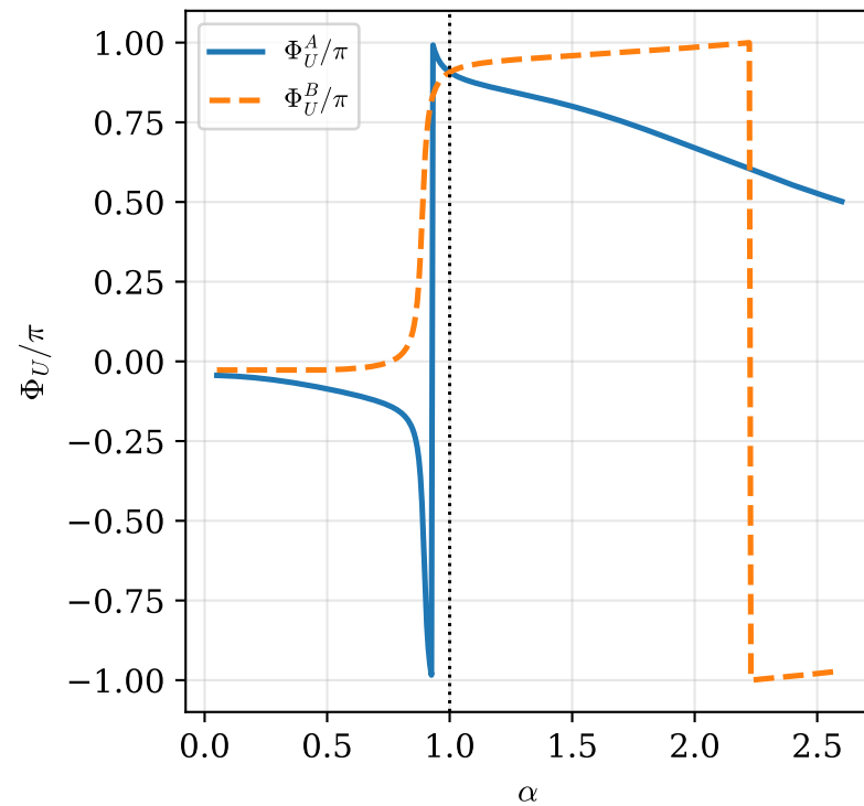
(b) the phases follow the populations
