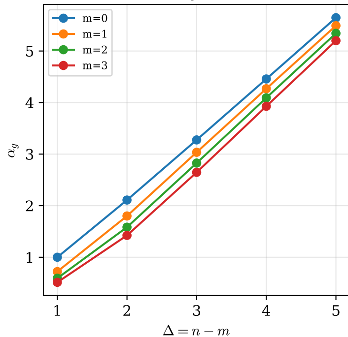
(c) \alpha_g vs \Delta
