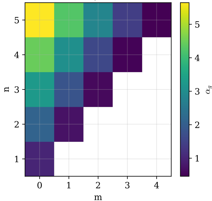
Critical overlap structure (b) \alpha_g(m,n)
