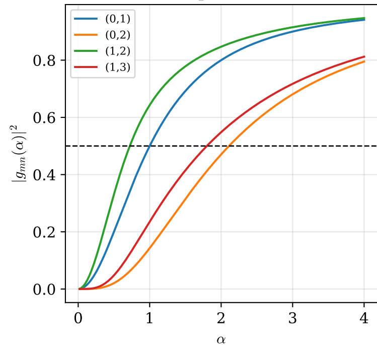
(a) overlap vs. threshold
