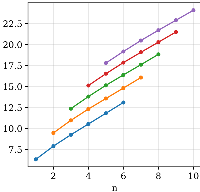
Global Berry phase vs. photon-addition indices ( n > m )
