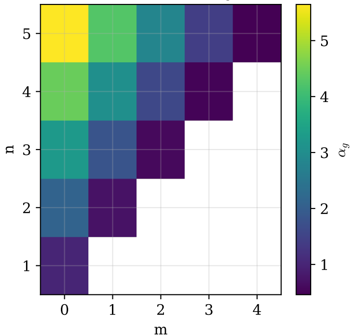
Critical overlap structure (b) critical function \alpha_g(m, n)
