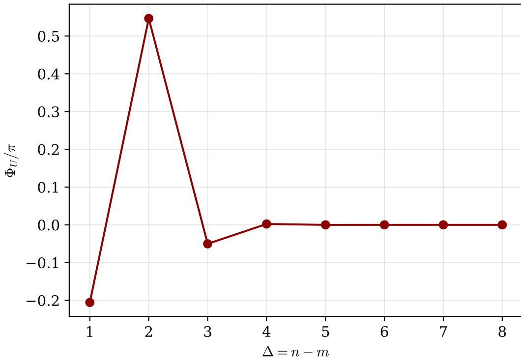
Uhlmann phase vs \Delta (balanced, m = 0 , \alpha = 1.2 )
