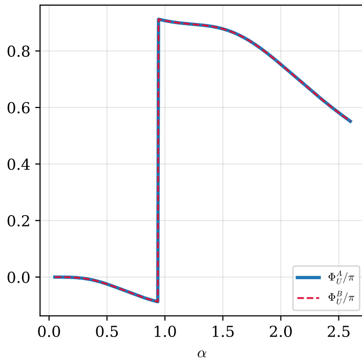
Uhlmann phase of BOTH subsystems under the global cycle ((m, n) = (0, 2), \mu = 0.6)
