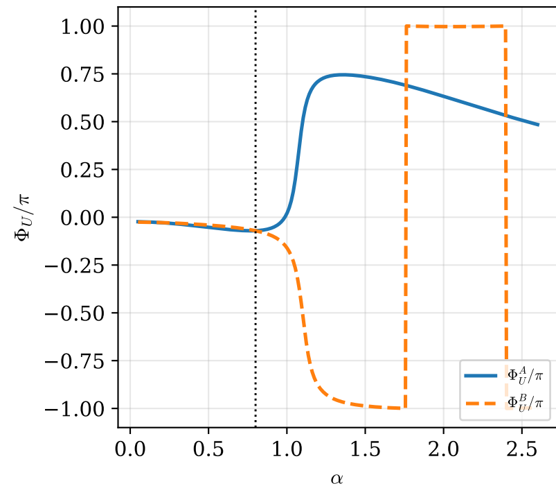
Uhlmann phase of BOTH subsystems under the global cycle ((m, n) = (0, 2), \mu = 0.6)
