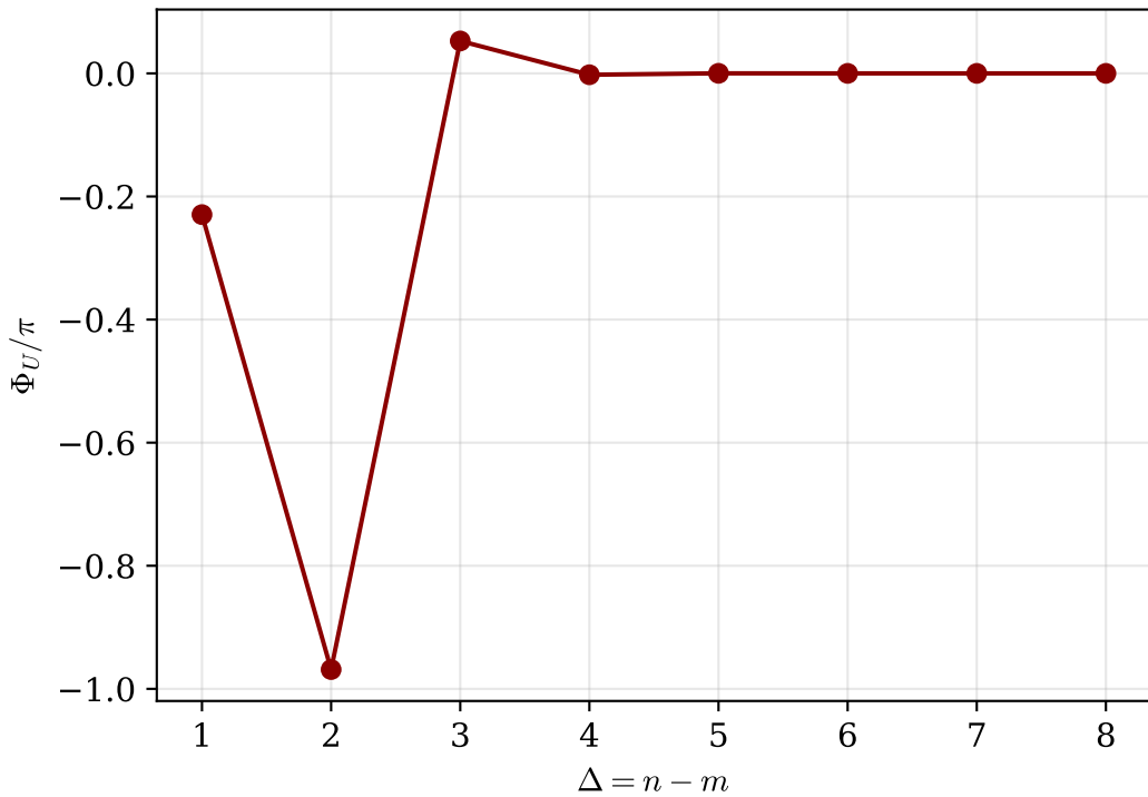
Uhlmann phase vs. \Delta , m = 0 , \alpha = 1.2
