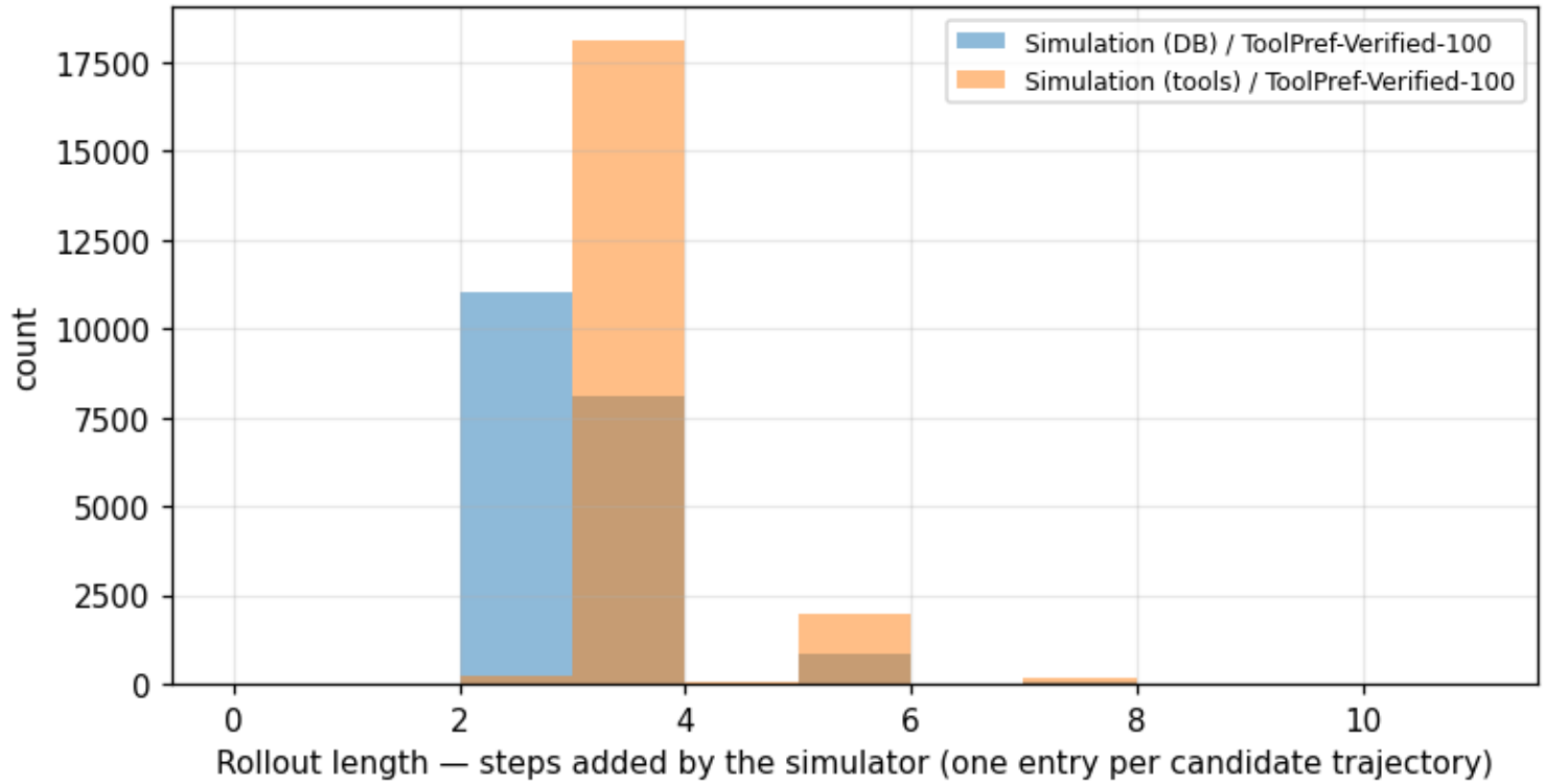
Rollout length distribution (simulation methods)
